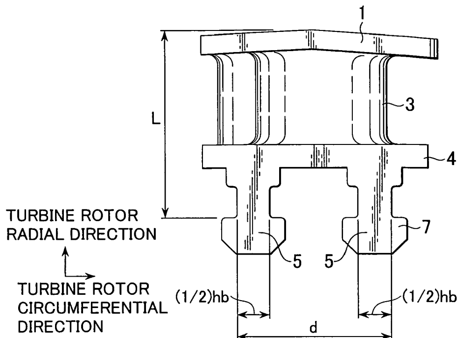
FIG. 7 SINGLE BLADE AND DUAL BLADE ROOT
