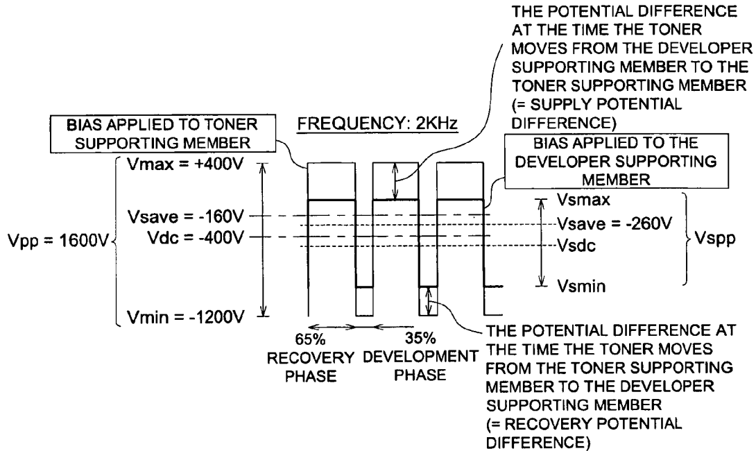
FIG. 5 ( a ) WHEN V_{spp} IN TABLES 1 TO 8 IS "+"
