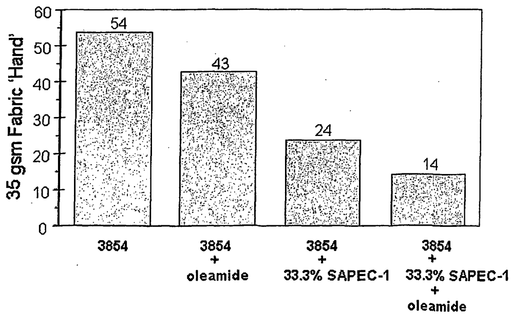
Figure 4: Nonwoven fabric Hand for Example 4-1 vs ACHIEVE 3854 control
