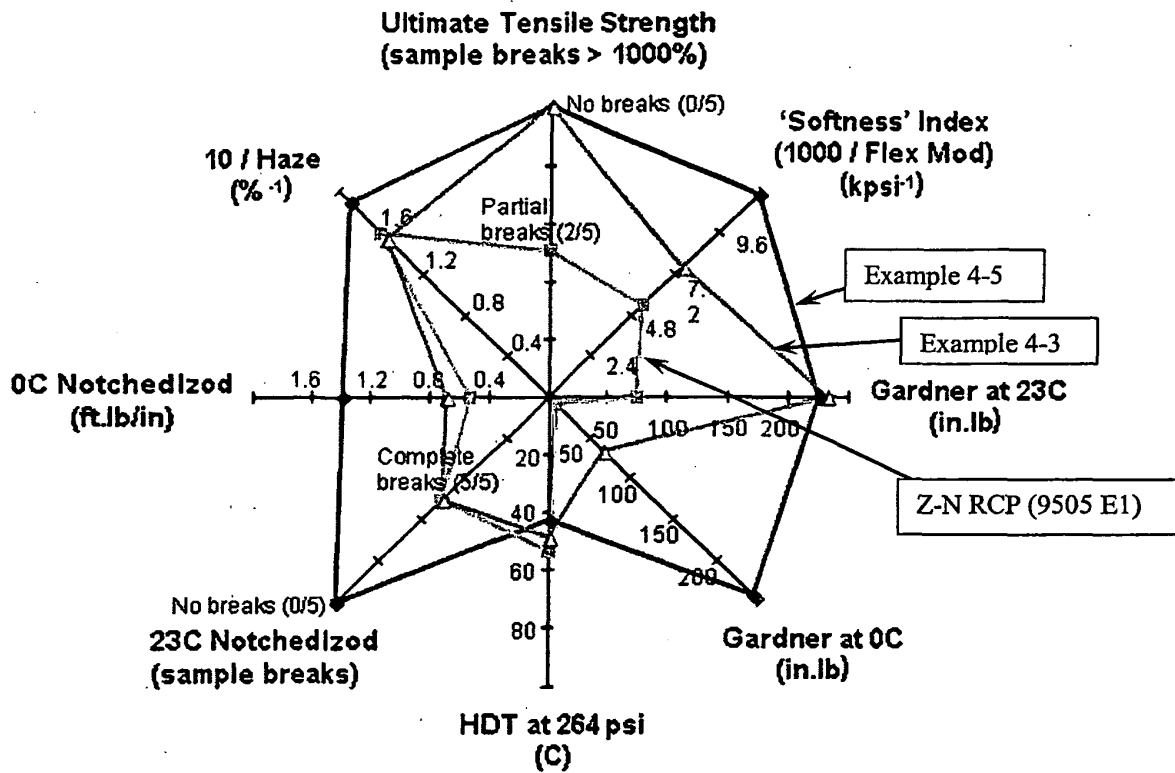
Figure 3: Molded-part properties Comparison of Examples 4-3 and 4-5 with Commercial Z-N random copolymer
