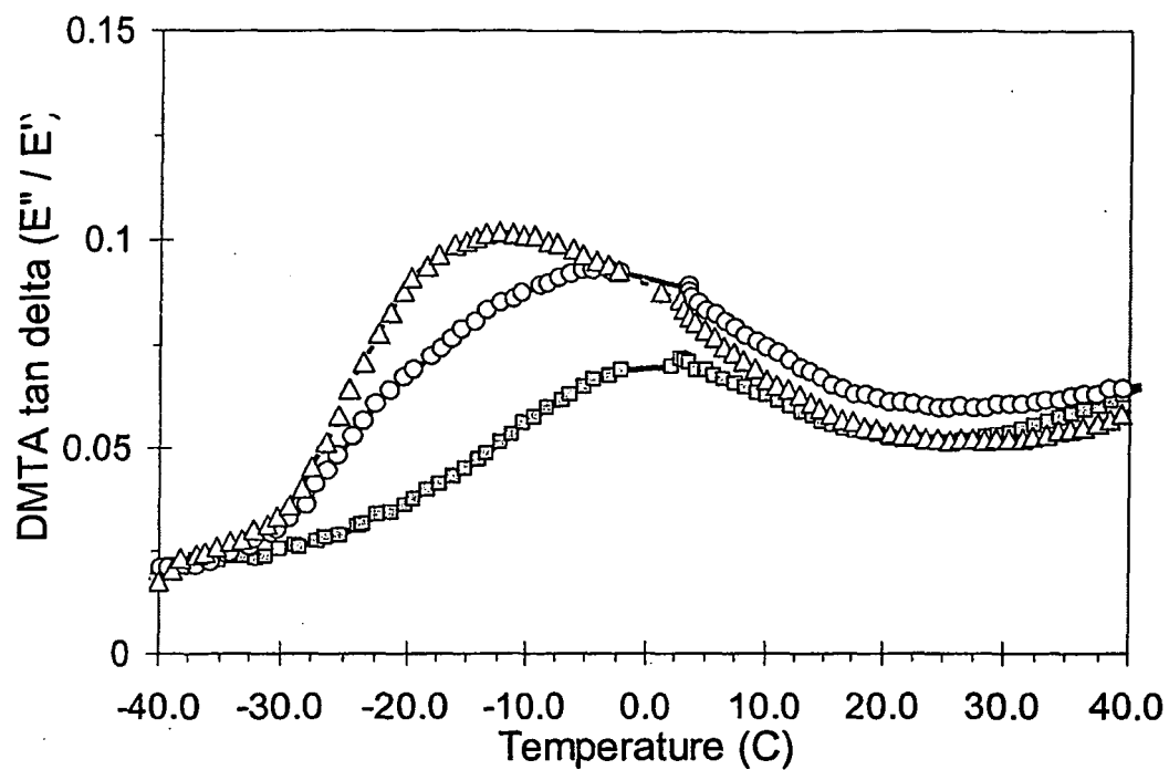
Figure 1: DMTA \tan \delta ( E''/E' ) for Homogeneous Blend Examples 4-2, 4-3, 4-5
