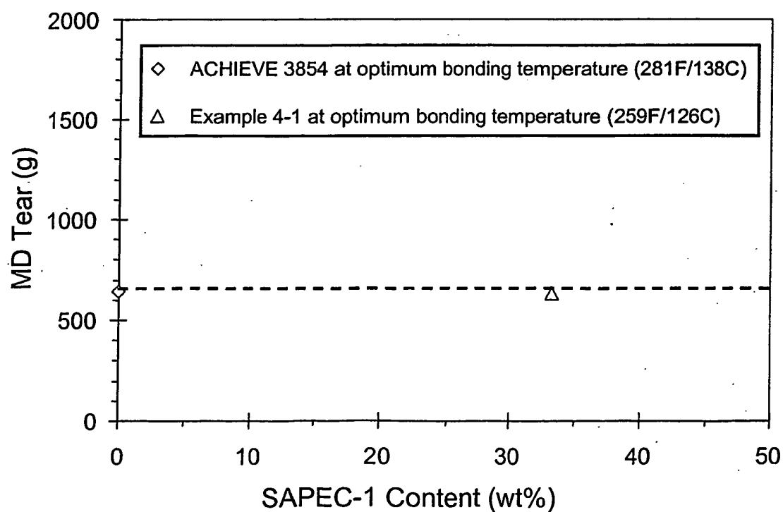
Figure 6: MD Tear resistance (35 g/m 2 fabrics) for Example 4-1 & 3854 control
