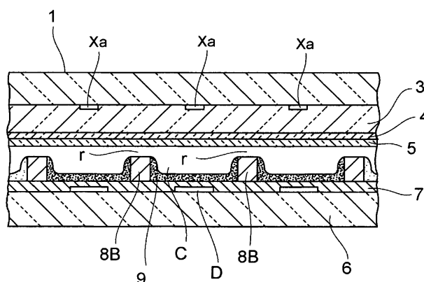
SECTION W-W
