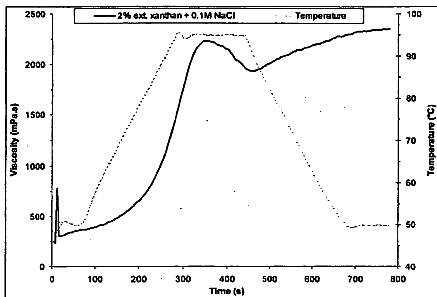
Figure 1. Temperature and Viscosity Profile of Particulate Xanthan in Rapid Viscosity Analyser
