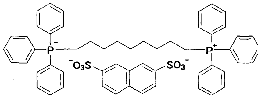
Phosphonium compound (1):
