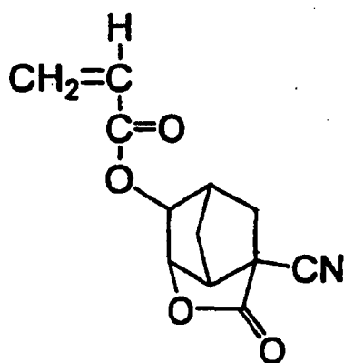
monomer-1
