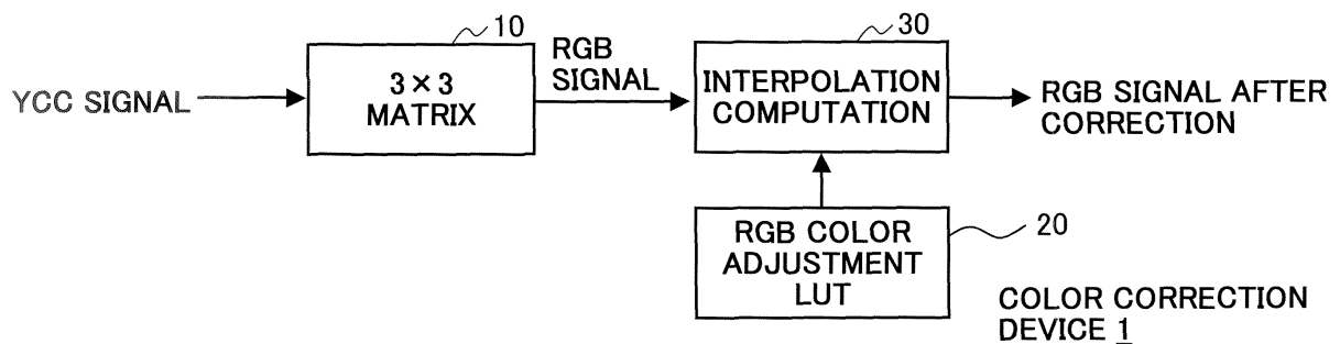
FIG. 1A CONFIGURATION EXAMPLE OF COLOR CORRECTION DEVICE
