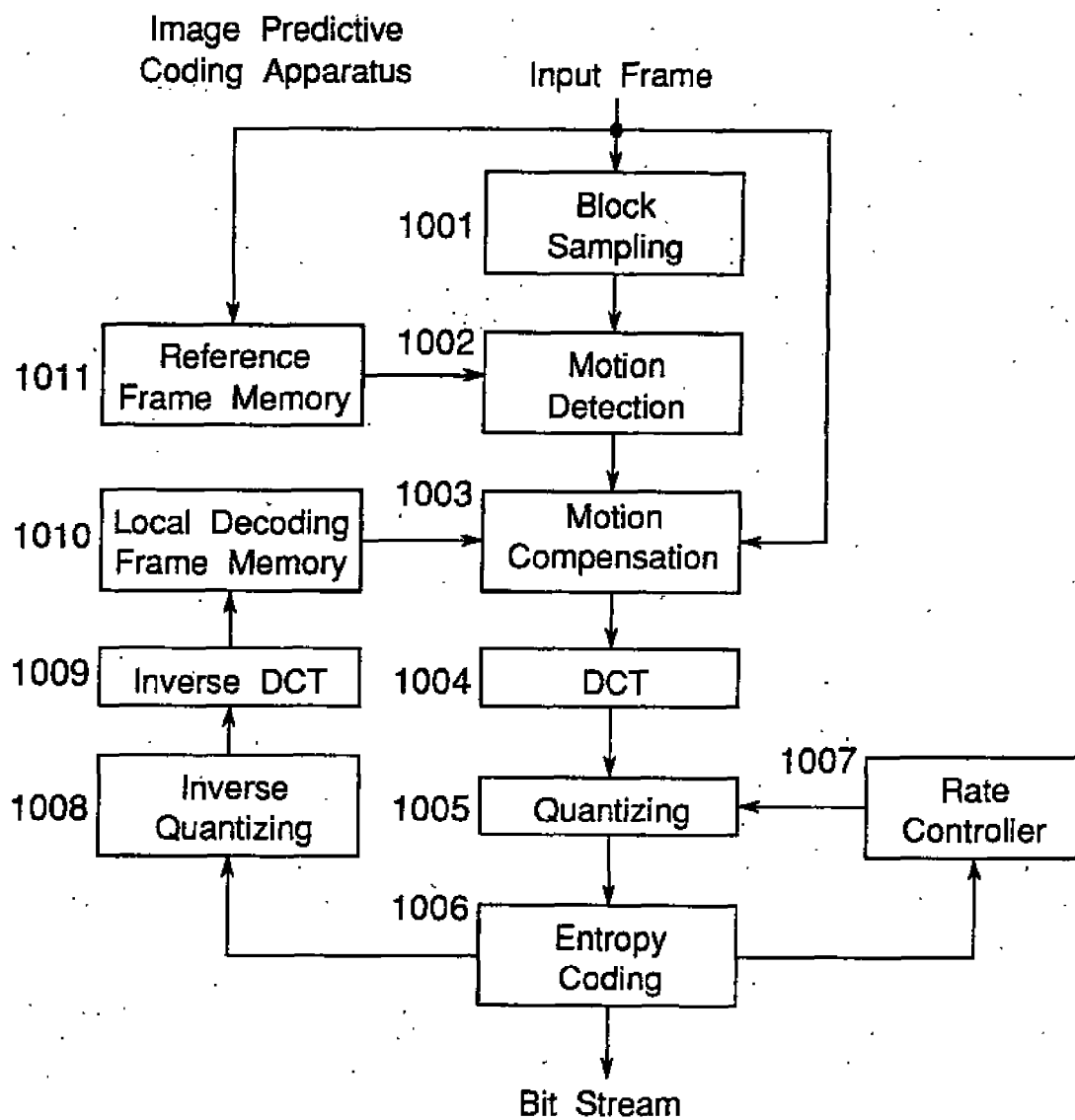
Fig.14 PRIOR ART
