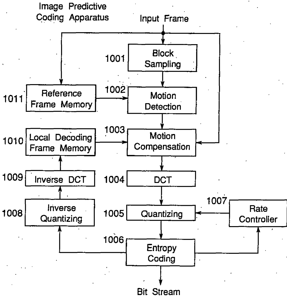
Fig.14 PRIOR ART
