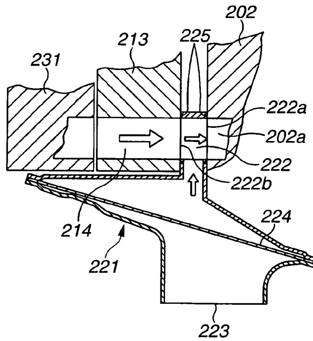
FIG.8 (PRIOR ART)
