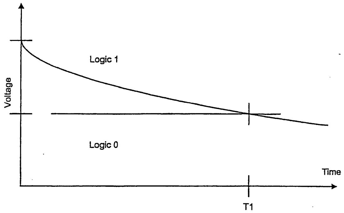
Figure 4(a): Discharge Waveform of Temporary Memory
