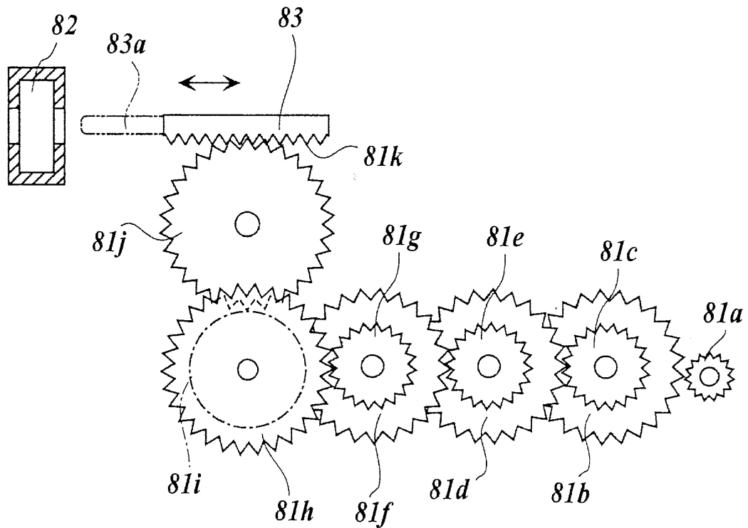
FIG 17B
