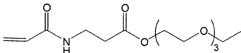
Example Compound 1
