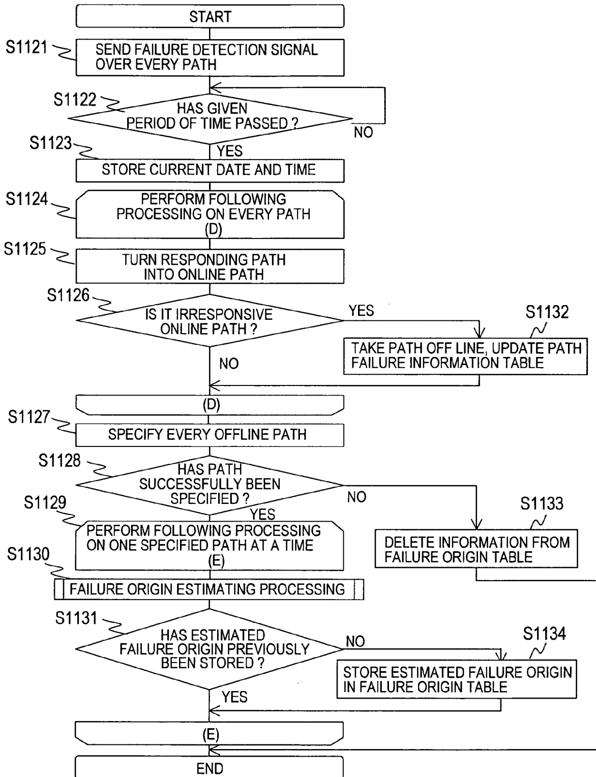
ALL-PATH FAILURE DETECTING PROCESSING
