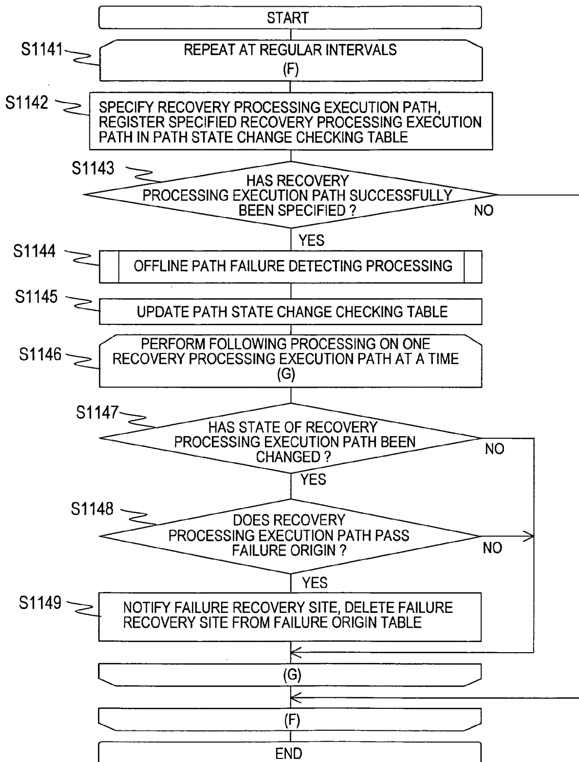
PATH FAILURE RECOVERY PROCESSING
