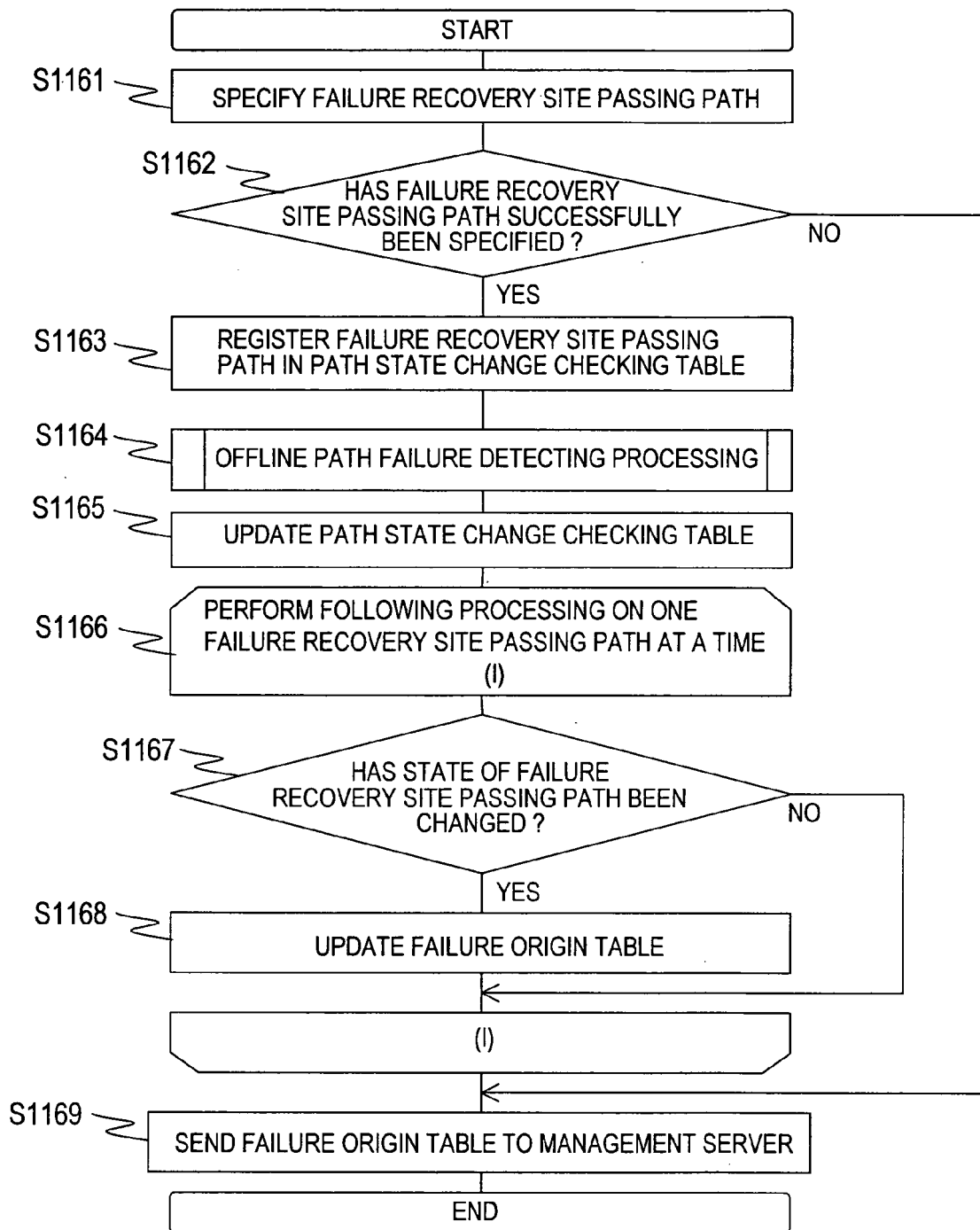
MANAGEMENT SERVER-PROMPTED FAILURE RECOVERY PROCESSING
