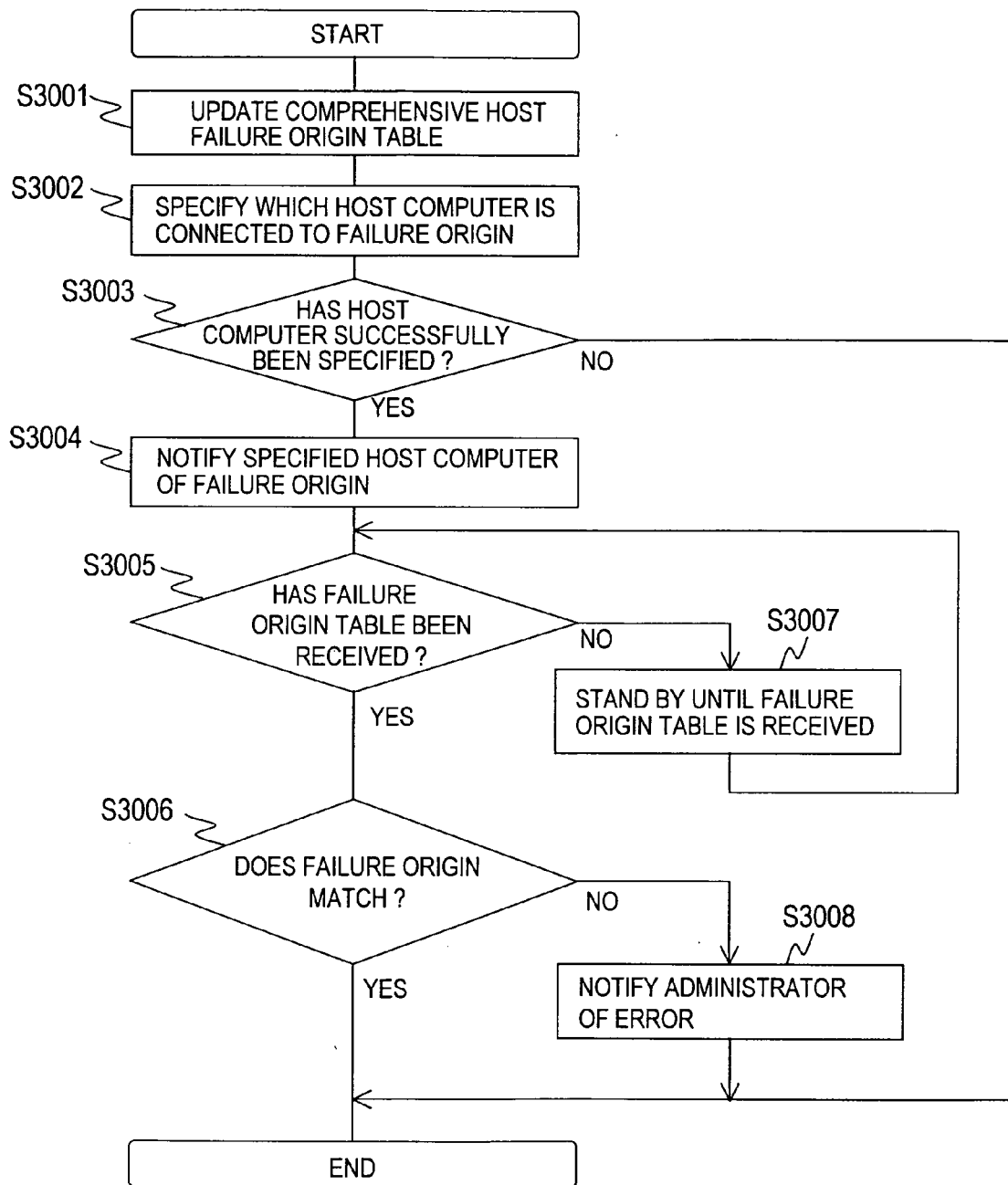
FAILURE ORIGIN CONFIRMING PROCESSING
