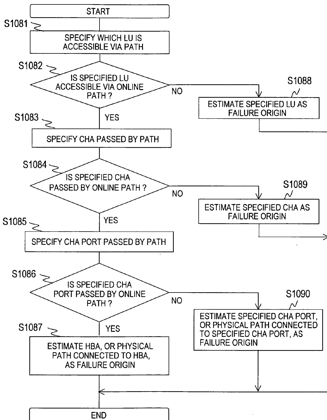
FAILURE ORIGIN ESTIMATING PROCESSING
