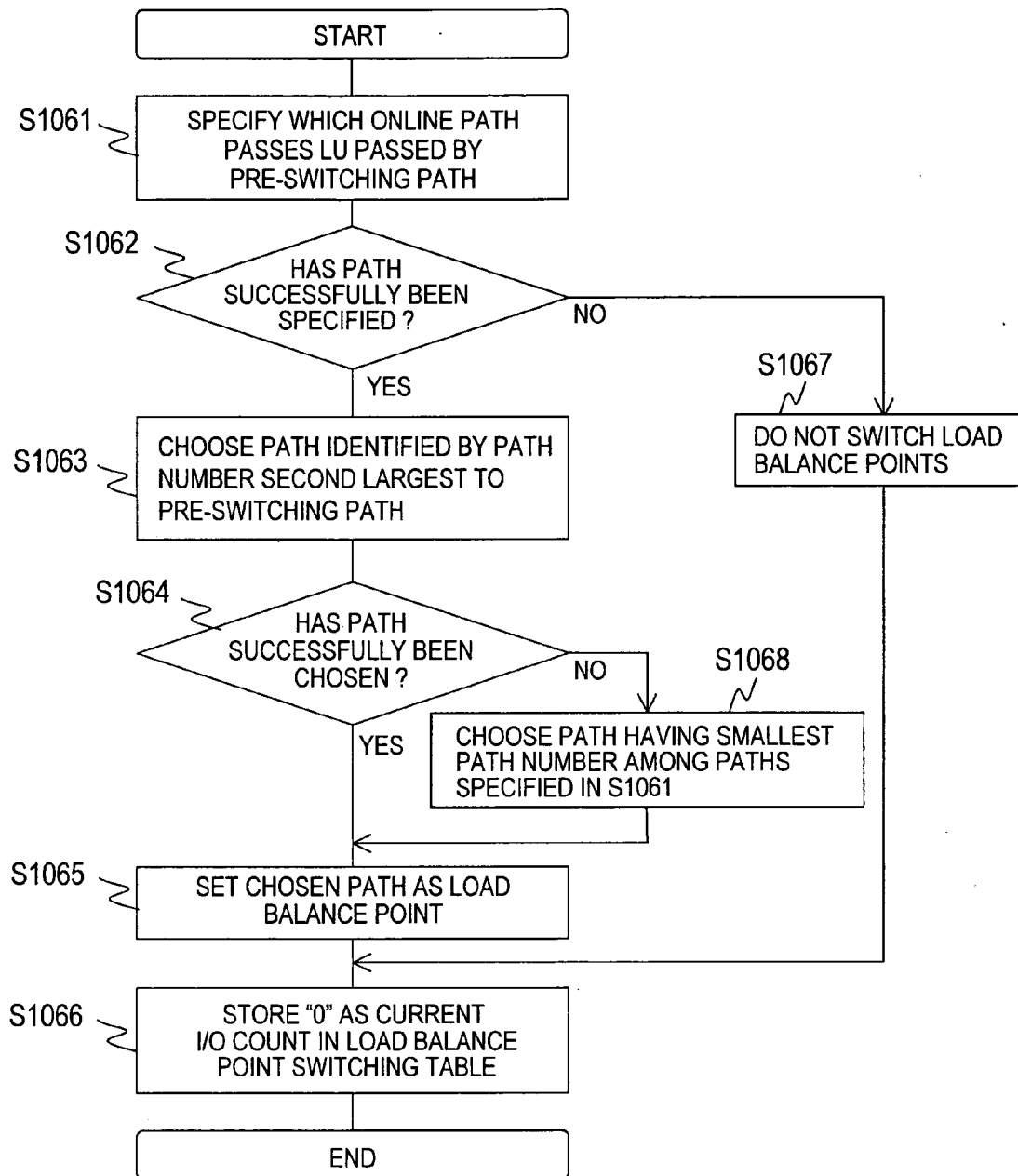
LOAD BALANCE POINT SWITCHING PROCESSING
