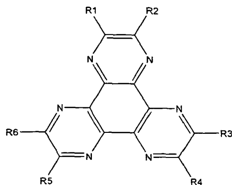
[0032] Formula I
