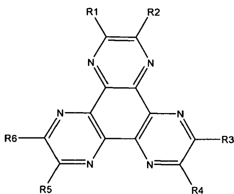
Formula I,
