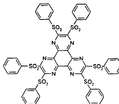
Formula Ib
