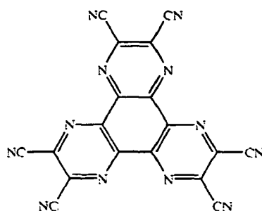
Formula Ia.
