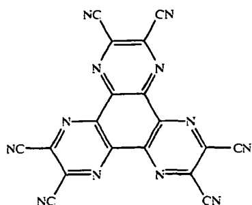
Formula Ia
