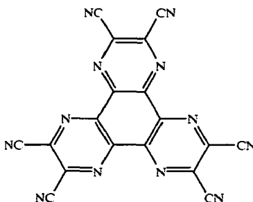
Formula Ia.
