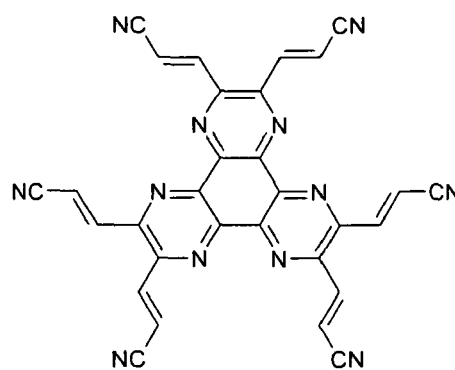
Formula If
