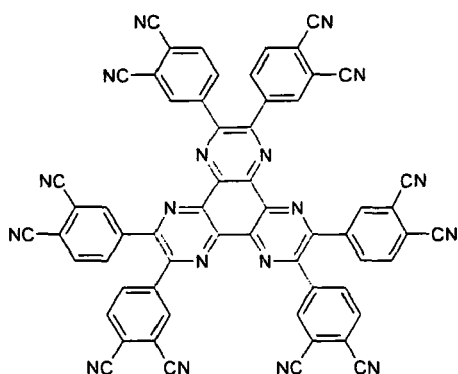
Formula Ie
