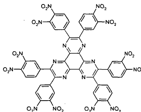
Formula Id
