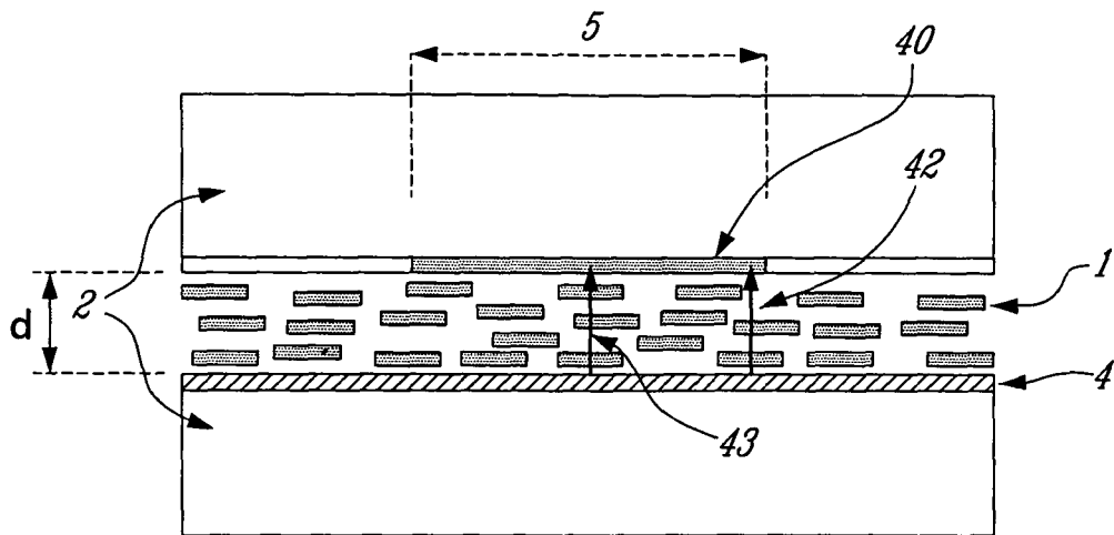
Fig. 2c (PRIOR ART)
