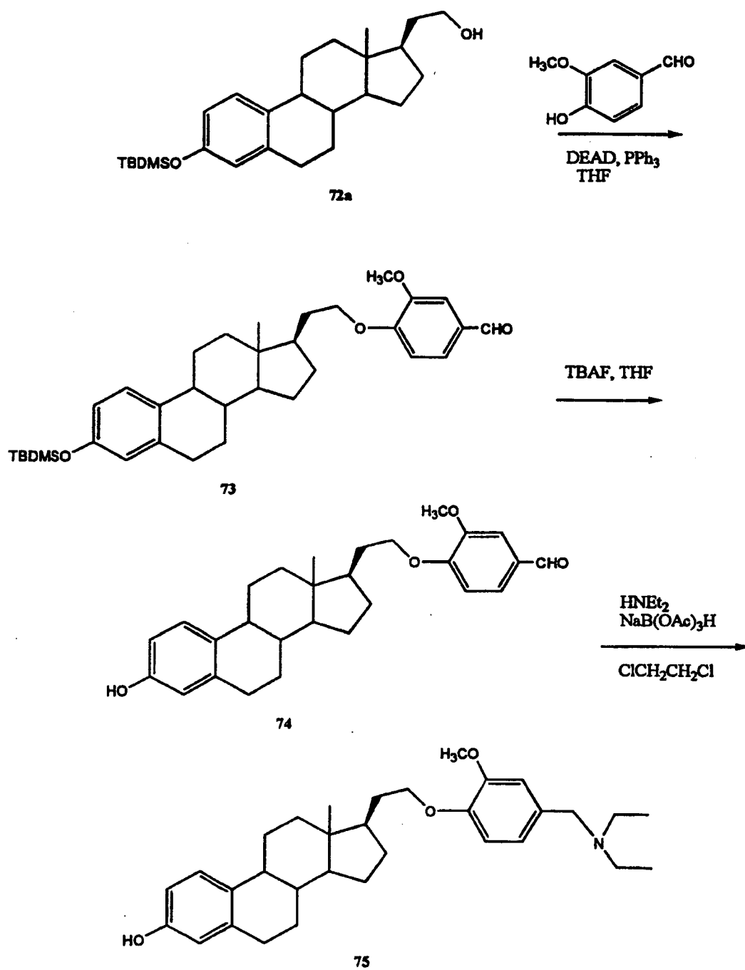
Scheme 15
