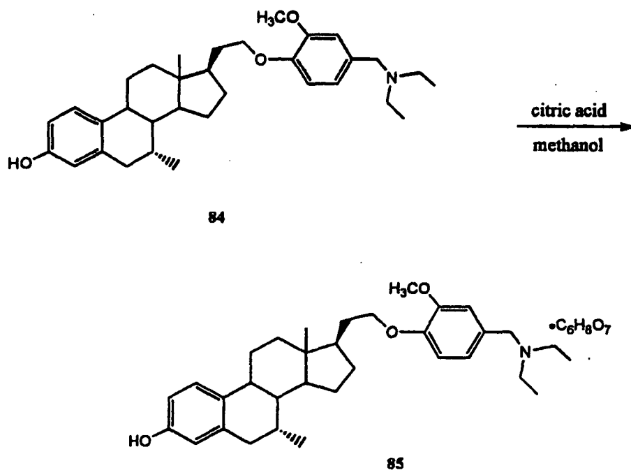
Scheme 18
