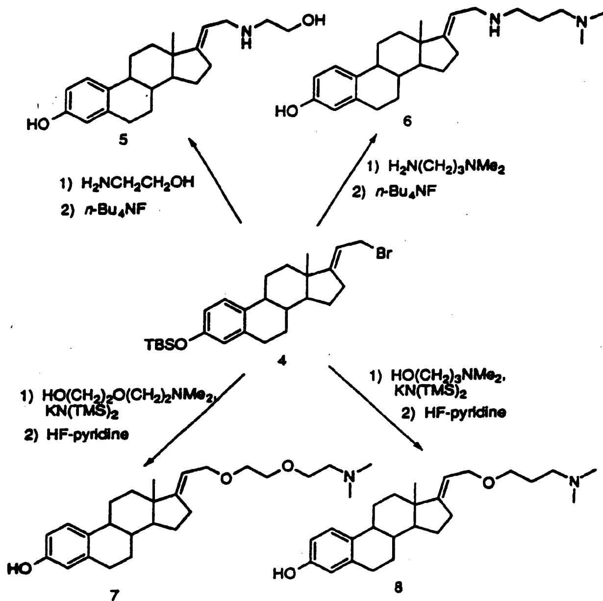
Scheme 2
