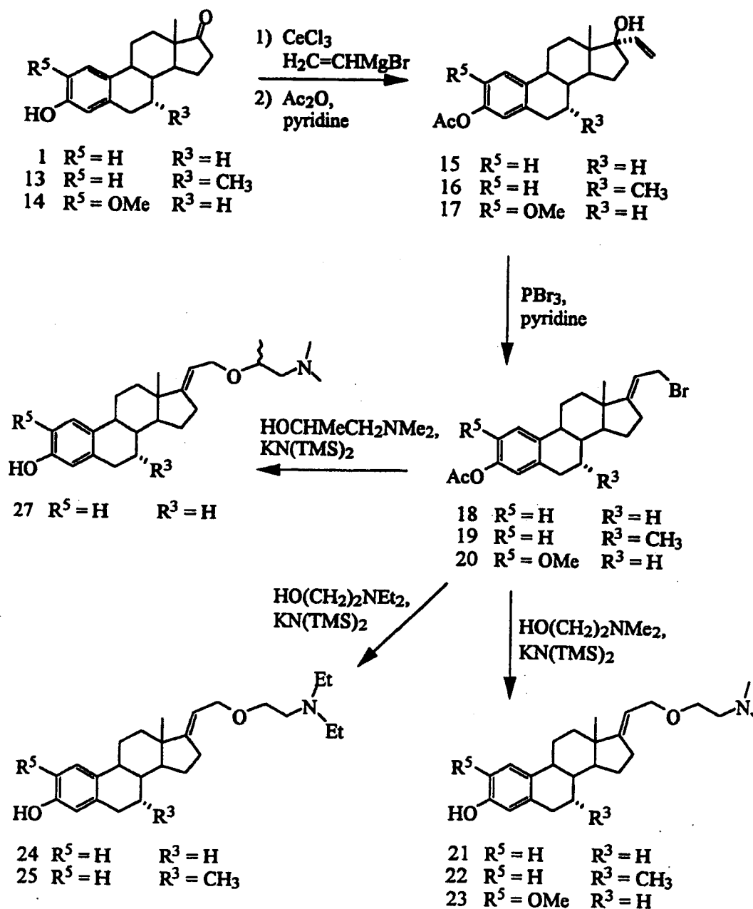
Scheme 4
