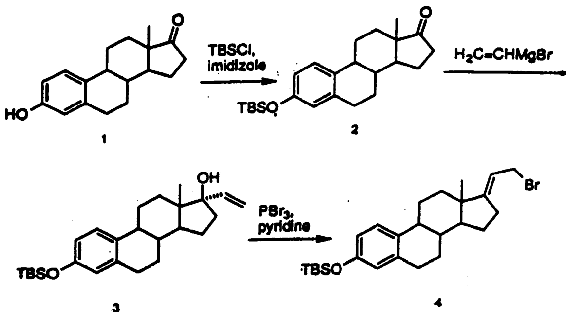
Scheme 1
