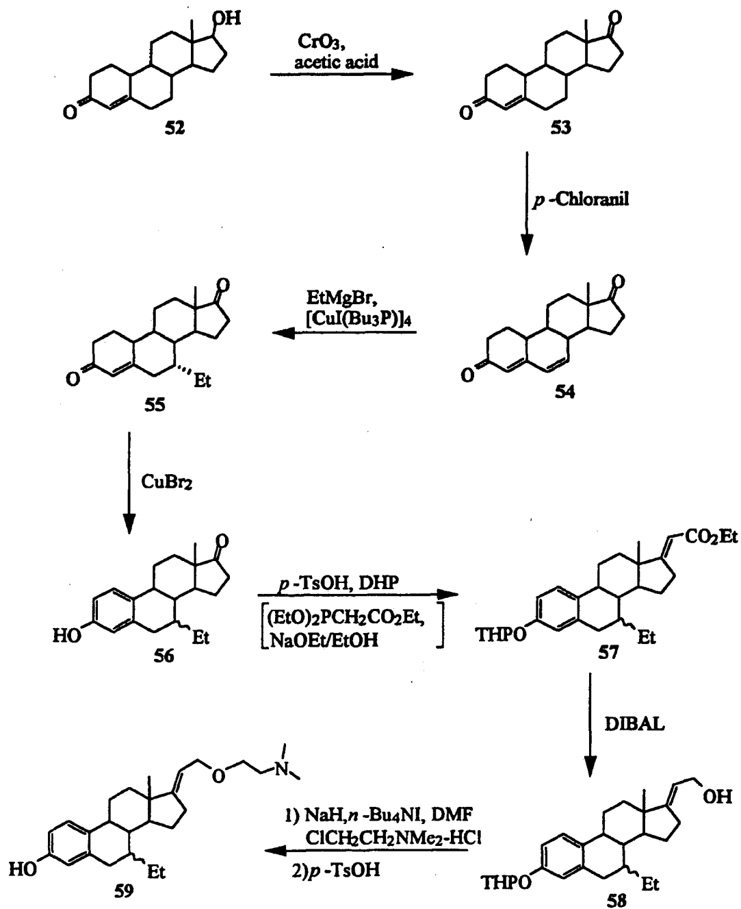
Scheme 11
