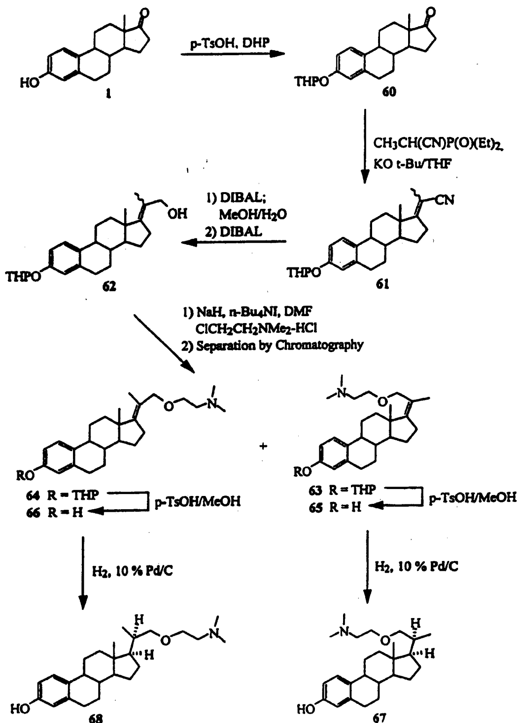
Scheme 12
