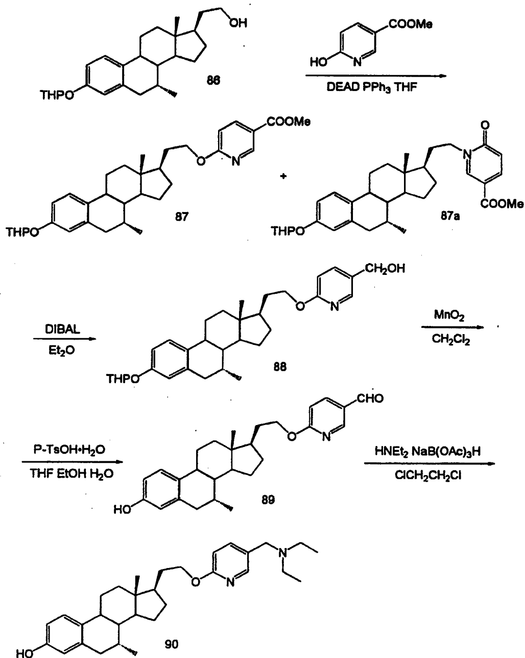
Scheme 19
