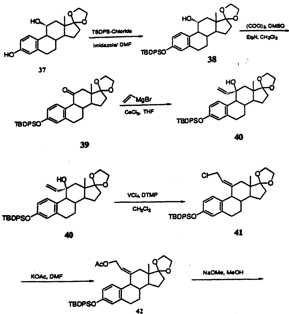
Scheme 8
