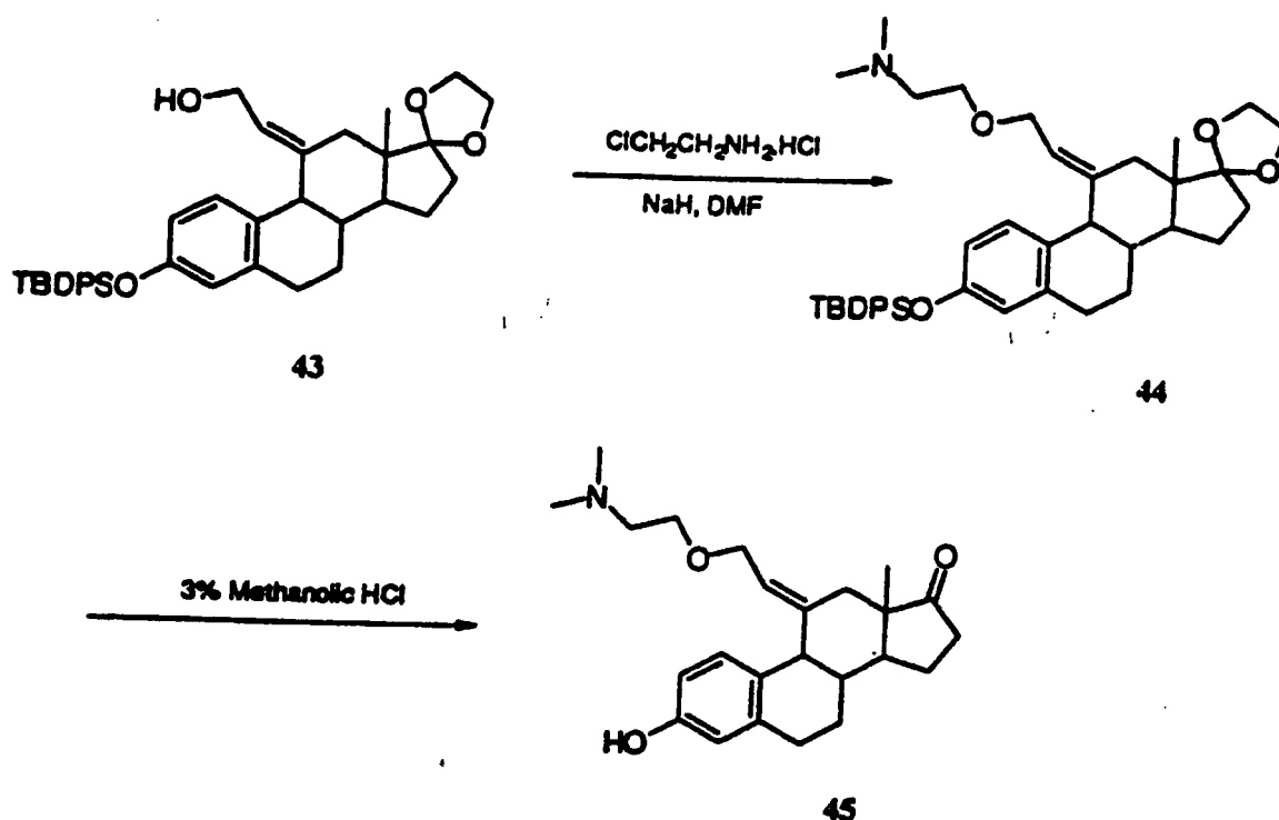
Scheme 8, continued
