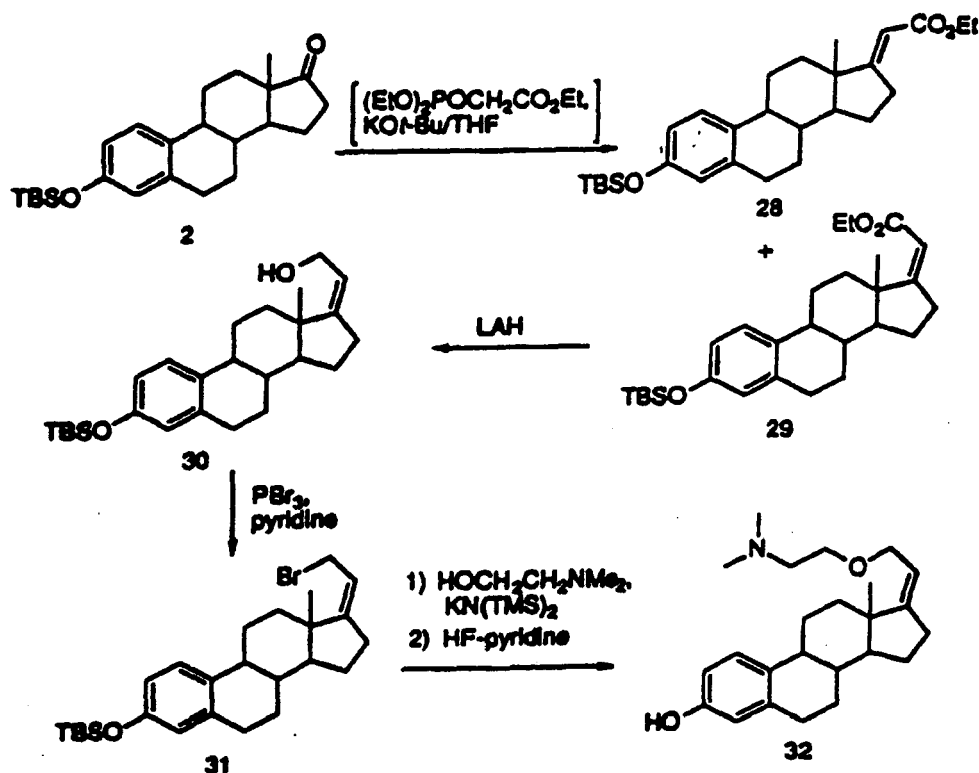
Scheme 5
