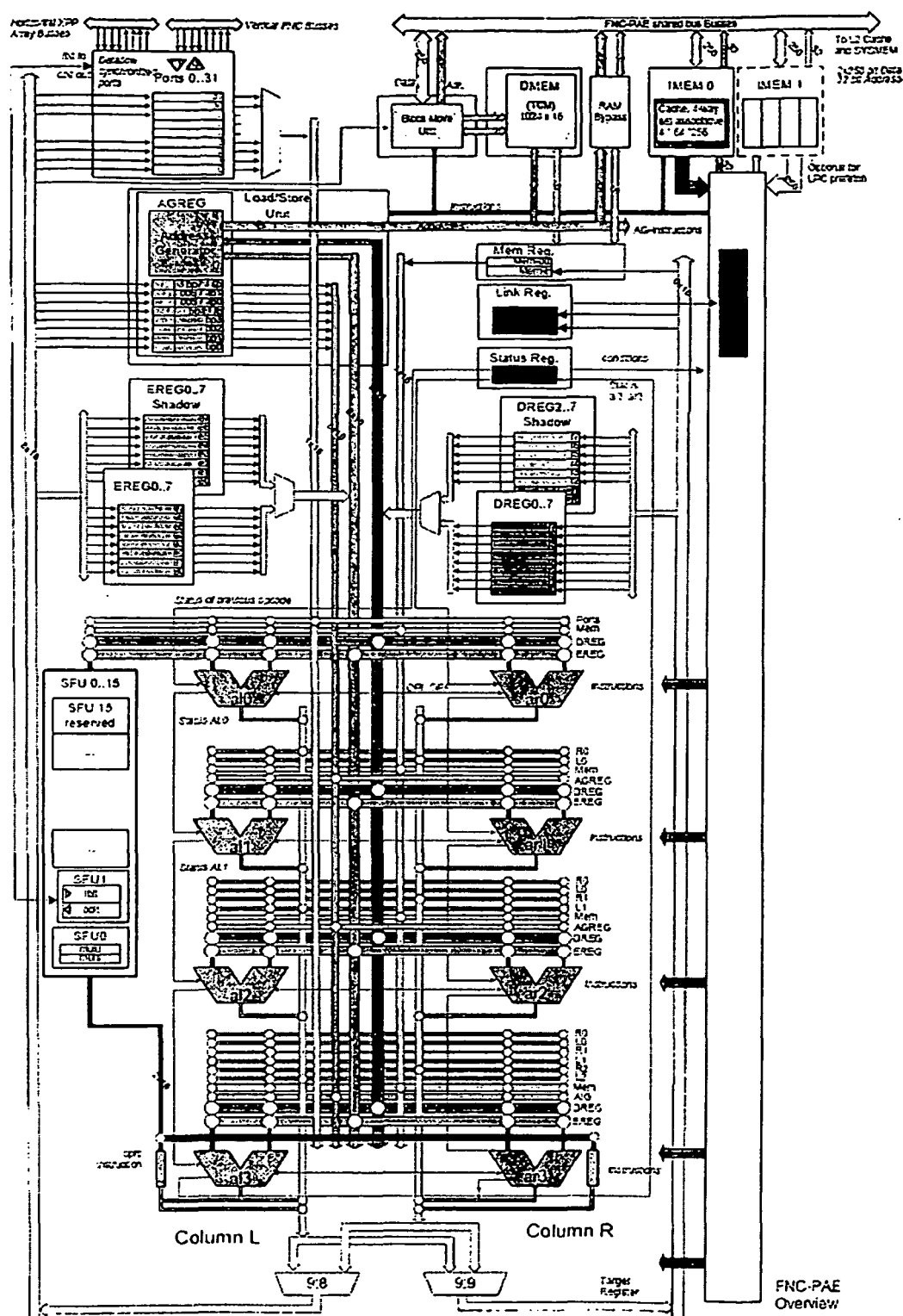
Attachment 1/Fig. 2: FNC-PAE Overview
