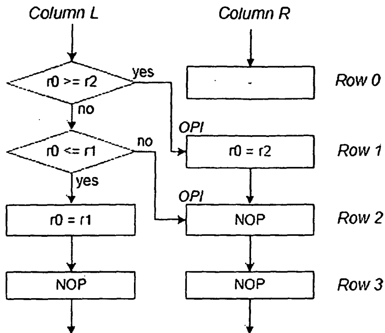
Attachment 1/Fig. 7: The instruction level flow graph
