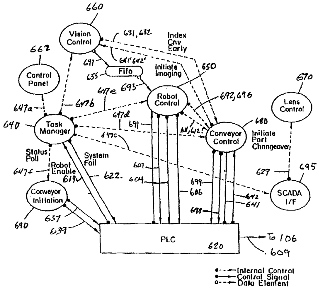
Fig. 8 : Needle Infeed System Task Diagram
