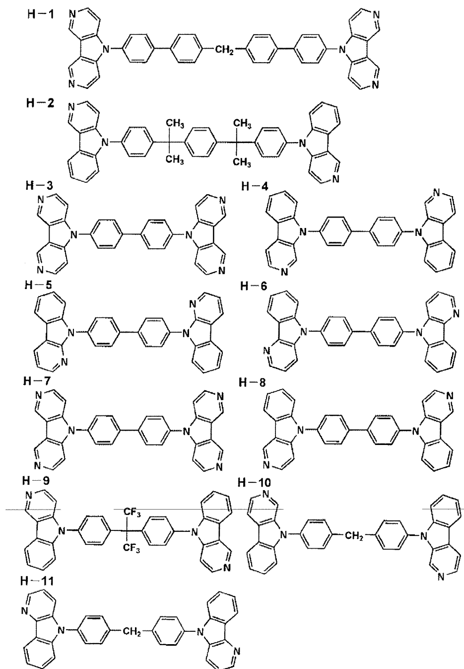
[Chemical Formula 4]
