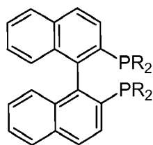
BINAP, R = aryl and alkyl
