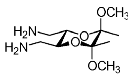
DioBD
