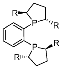
DUPHOS R = alkyl, alkoxy, hydroxy, amino, aryl
