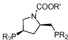
bpm R = Aryl, Alkyl R' = Alkyl
