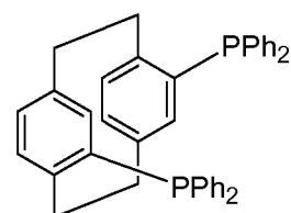
PHANEPHOS
