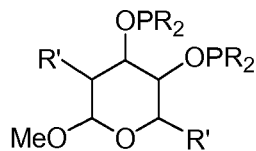
CARBOPHOS R = aryl R' = CH 2 C(O)Ph
