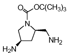
PyrBD
