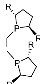
BPE R = alkyl
