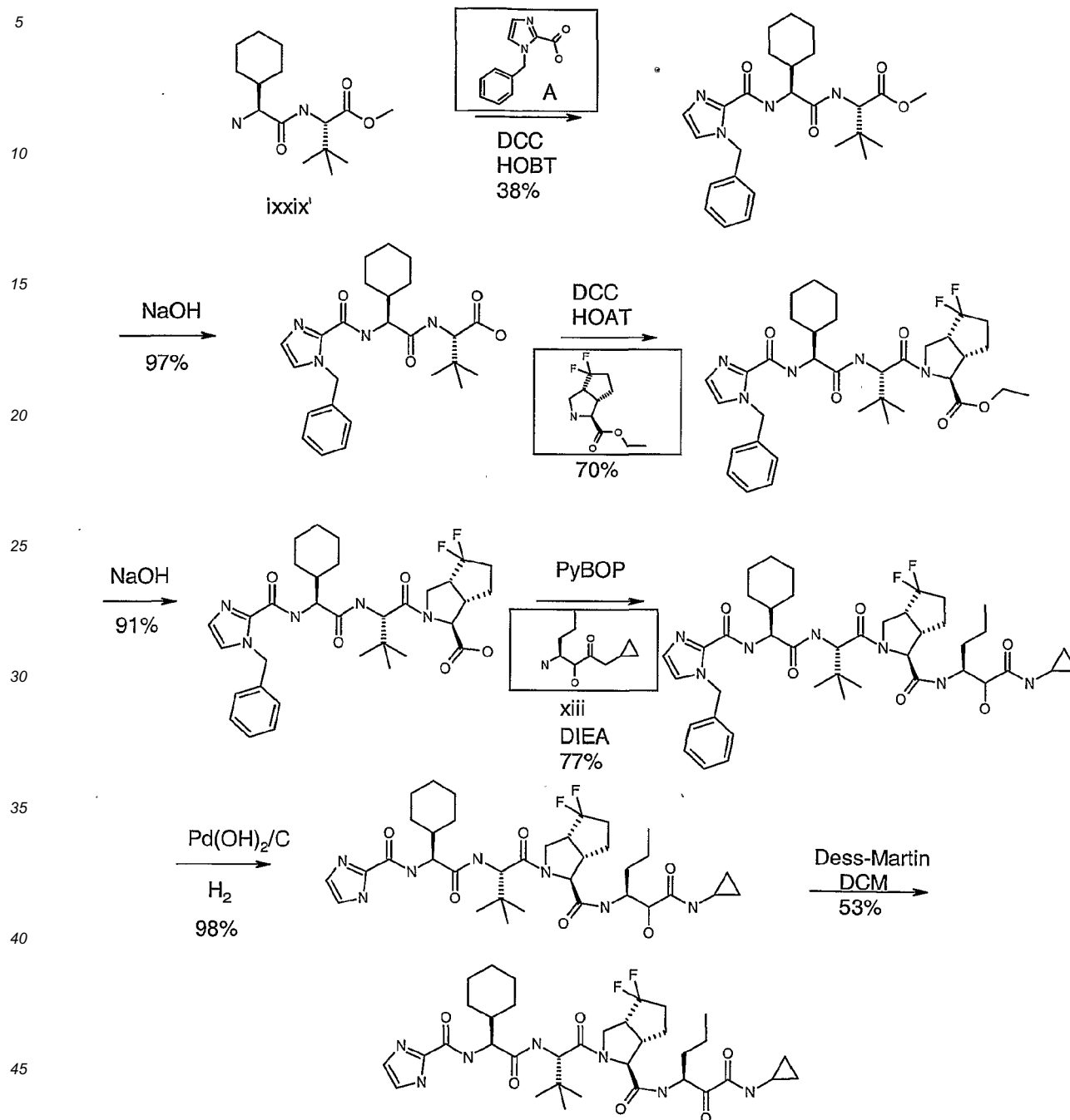
Scheme 11
