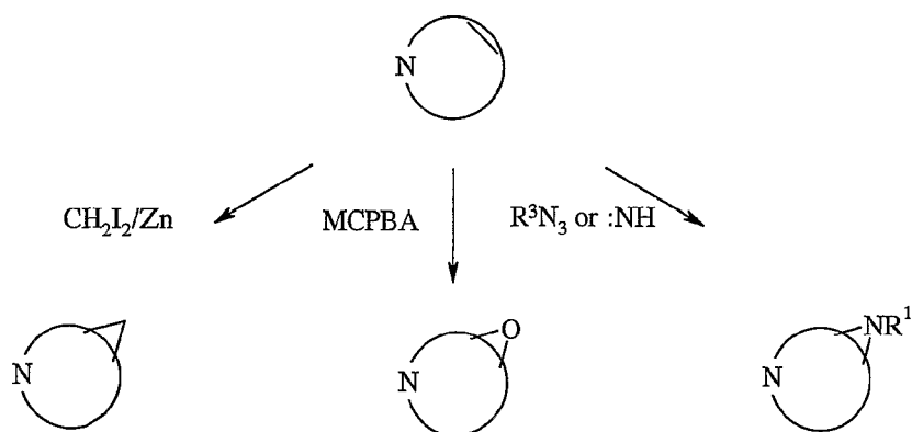
SCHEME 8
