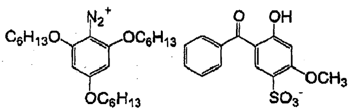
Electron Accepting Compound (2)
