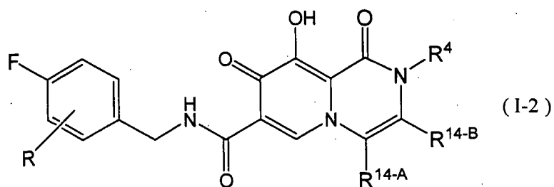
[Chemical formula 75]
