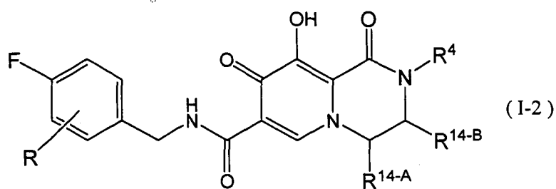
[Chemical formula 68]
