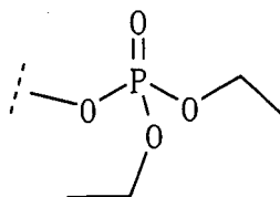
[Chemical formula 22]
