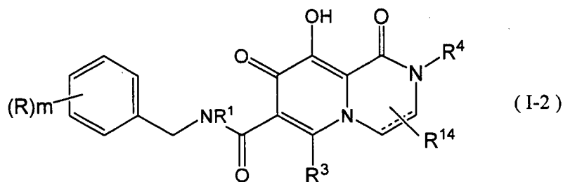
[Chemical formula 8]
