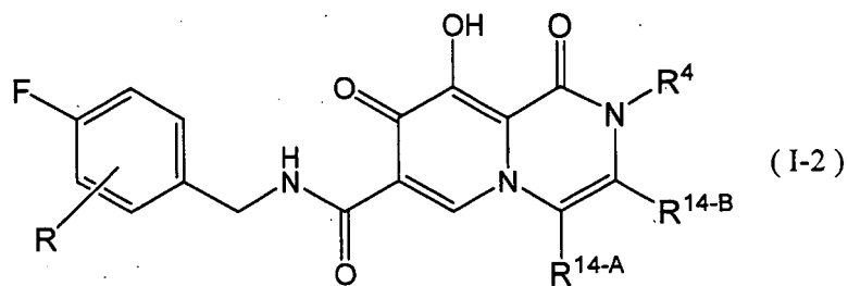
[Chemical formula 73]
