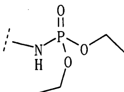
[Chemical formula 23]
