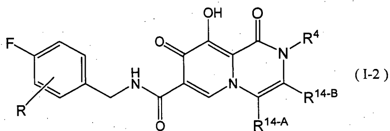
[Chemical formula 76]
