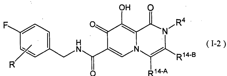
[Chemical formula 74]
