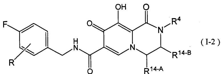
[Chemical formula 69]
