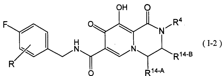
[Chemical formula 70]
