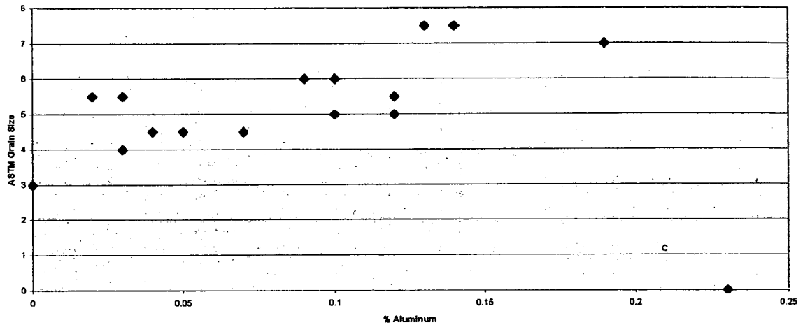
Figure 14 Effect of Al on Grain Size After Simulated Brazing Thermal Cycle
