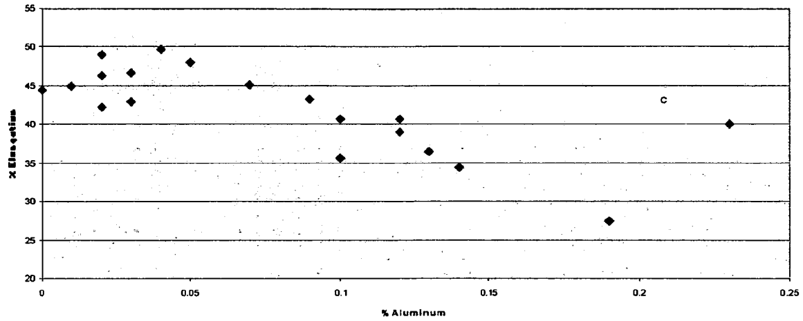
Figure 10 Effect of Aluminum on Ductility, 2000F Anneal
