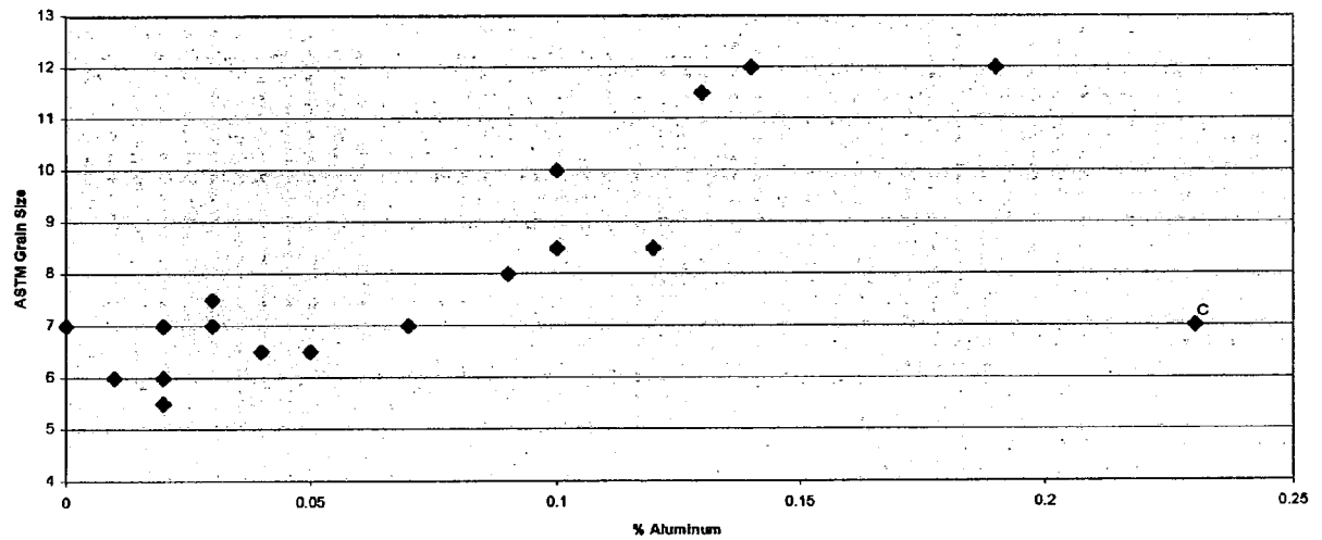
Figure 13 Effect of Al on Grain Size, 2000F Anneal
