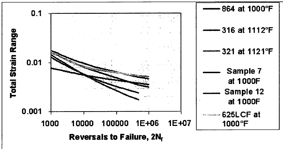
Fig. 17 High Temperature Fatigue Test Results – Longitudinal Strain Controlled
