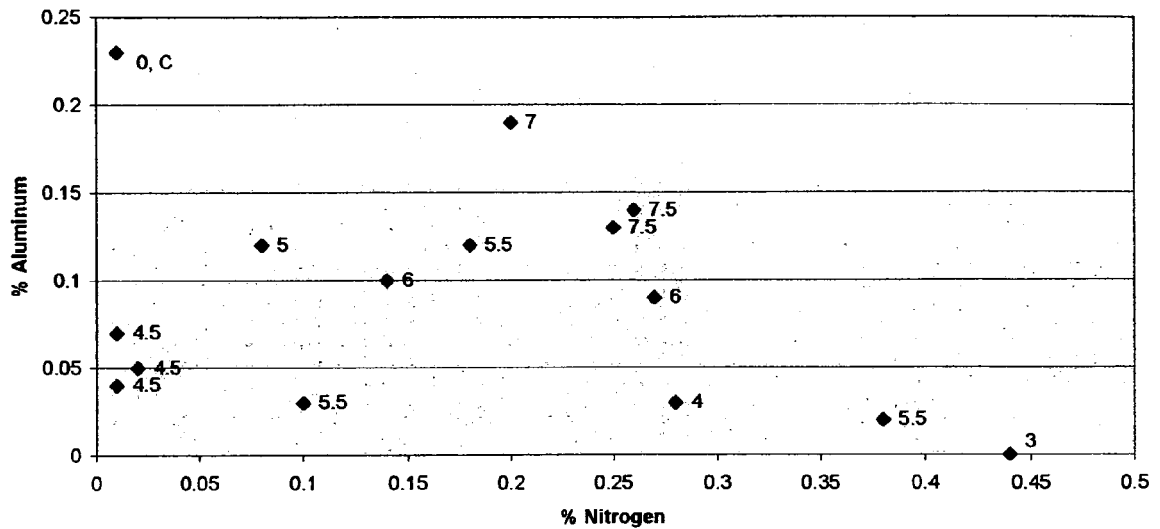
Figure 16 Effect of N and Al on ASTM Grain Size After a Simulated Brazing Thermal Cycle
