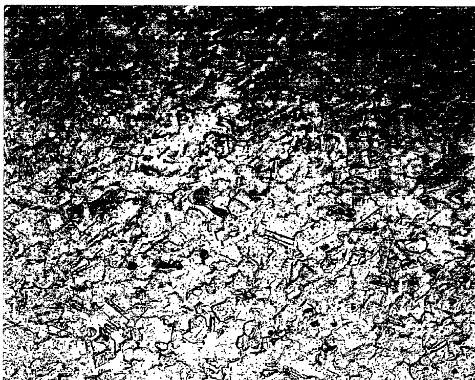
Fig. 3: Sample 7 (high Zr, N, Nb, Al) after 1800°F anneal, 500X, Br Etch
