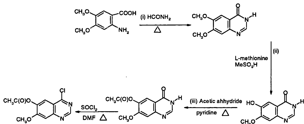
Reaction scheme 2
