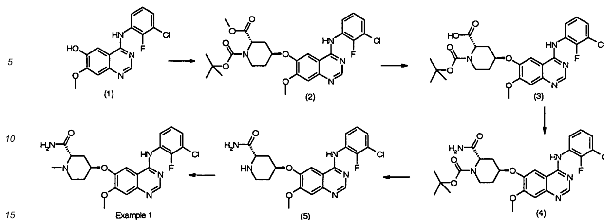
Scheme A
