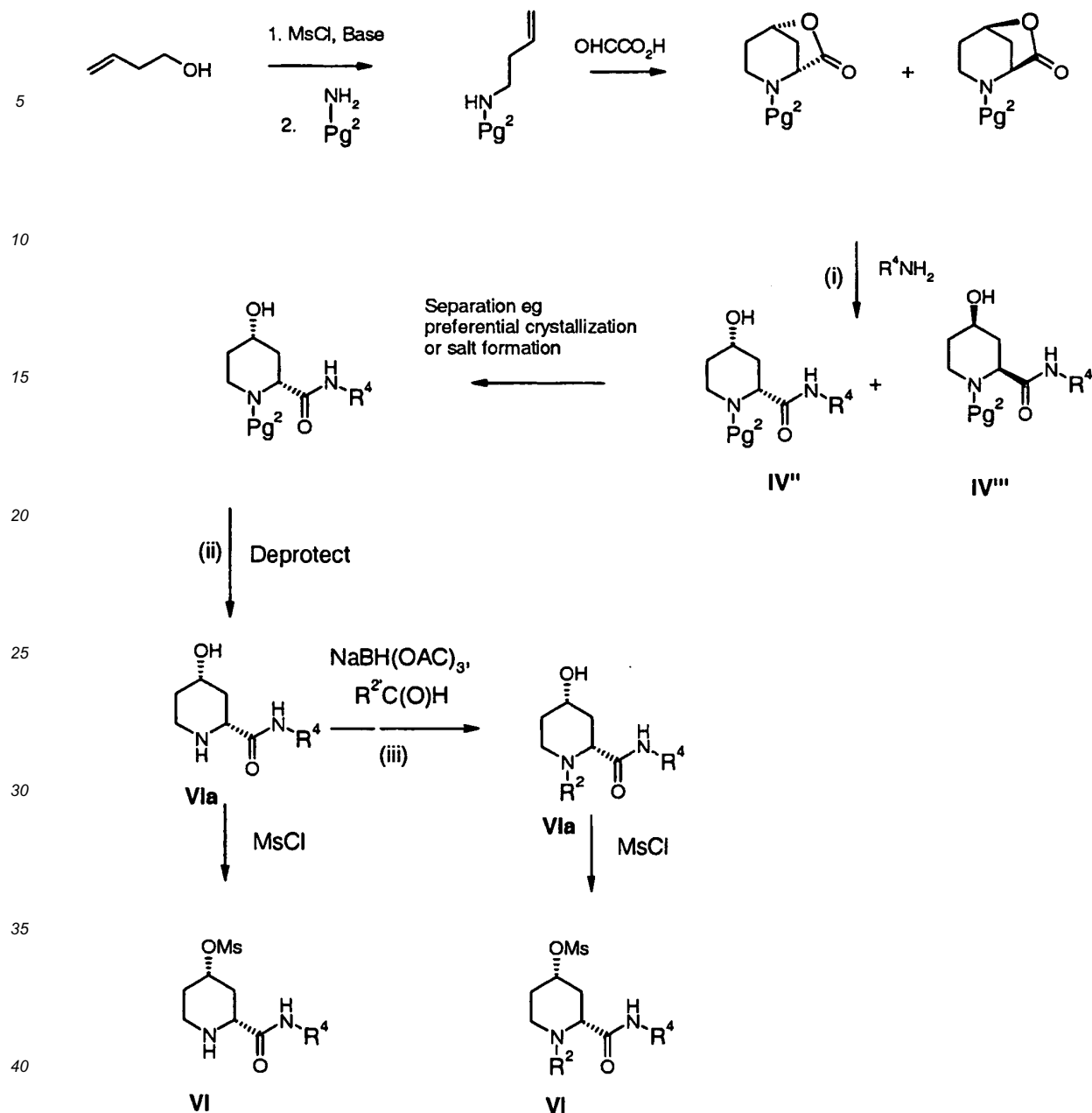
Reaction Scheme 4
