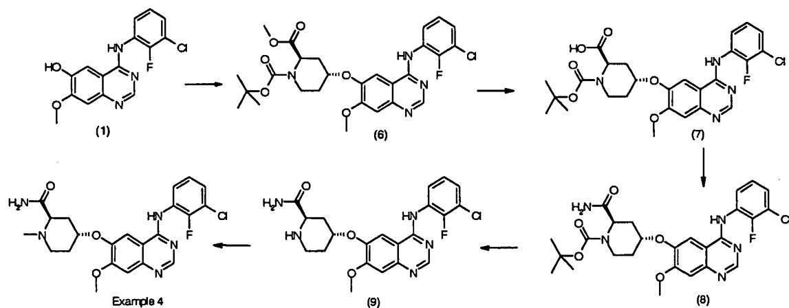
Scheme B
