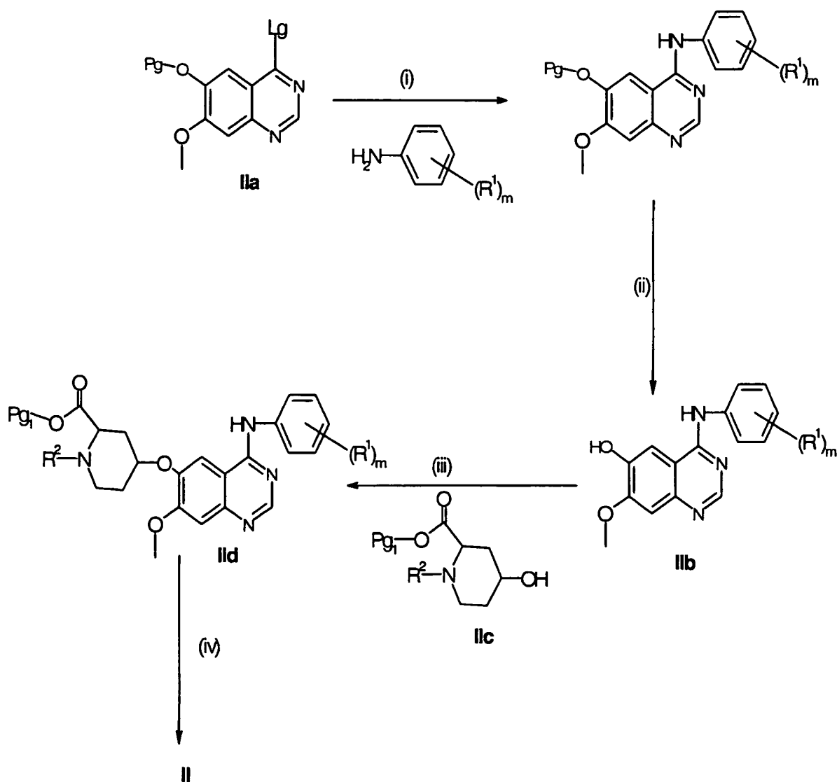
Reaction Scheme 1
