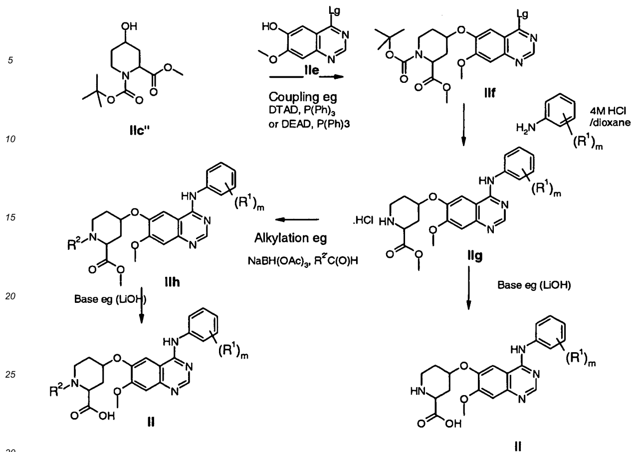
Reaction Scheme 1a:
