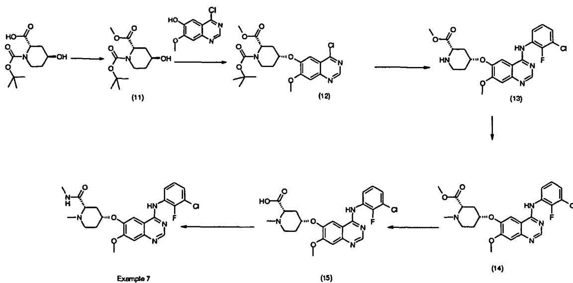
Scheme D
