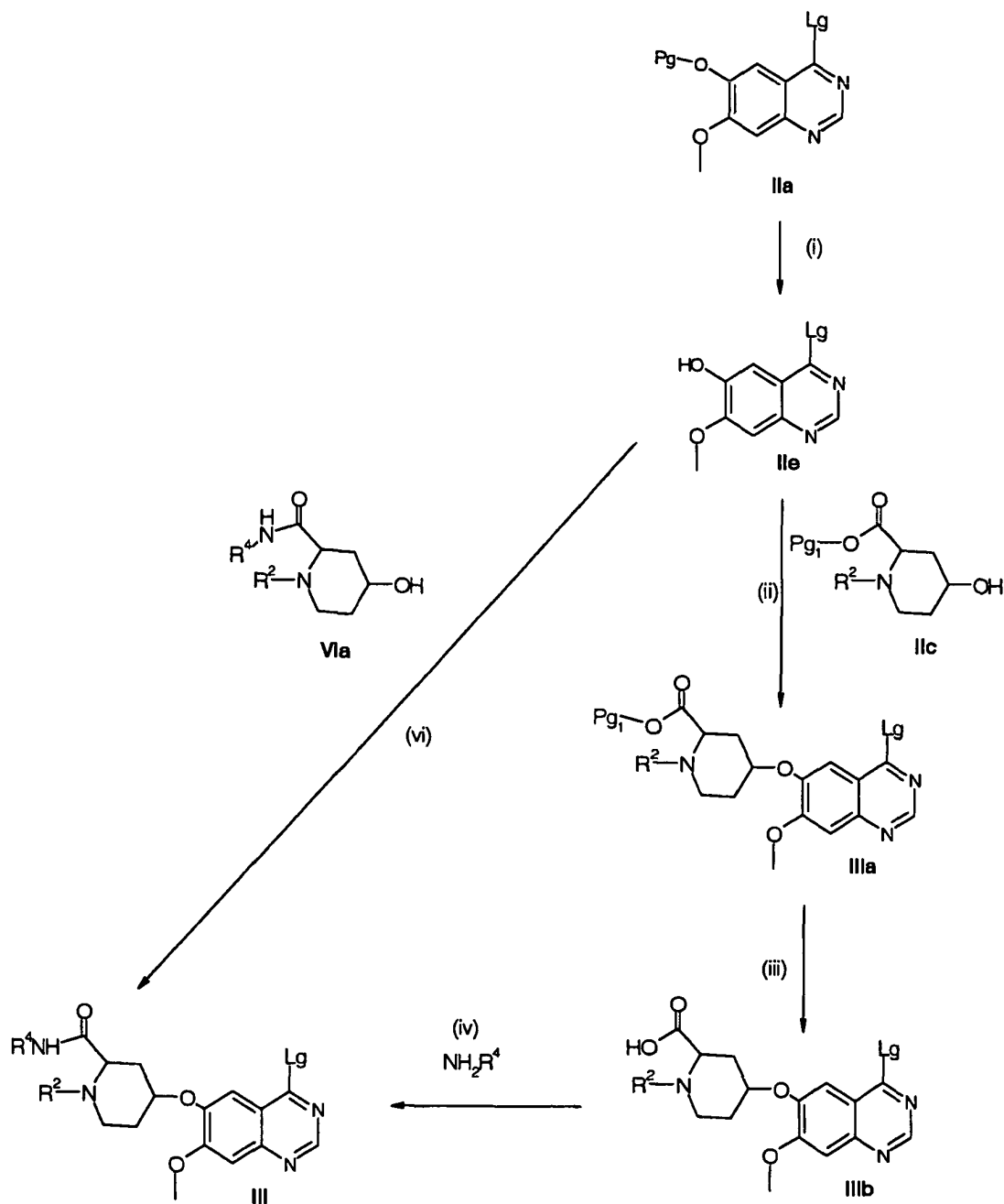
Reaction Scheme 3
