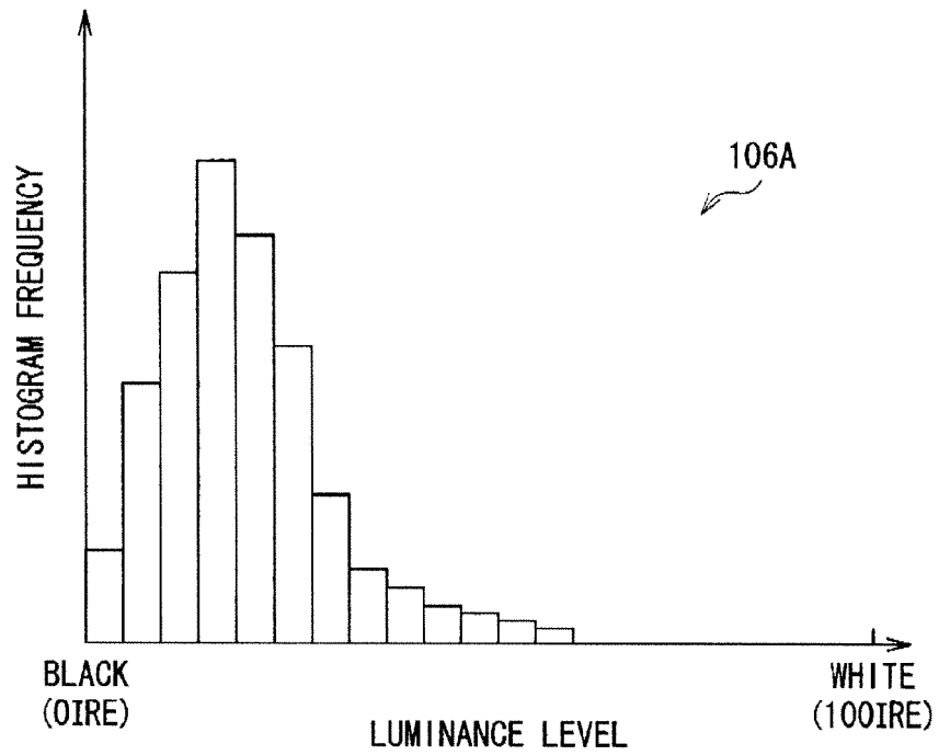
FIG. 13A RELATED ART
