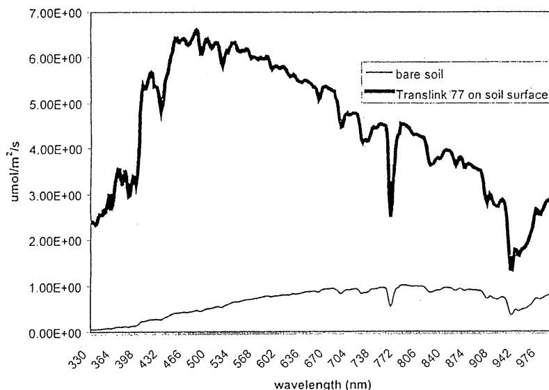
reflection spectra
