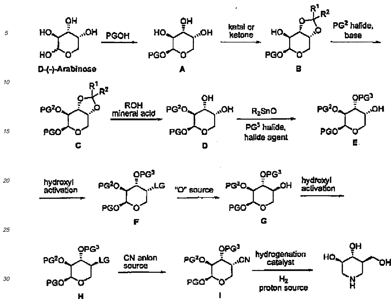
Scheme 1. PG is a protecting group; LG is a leaving group
