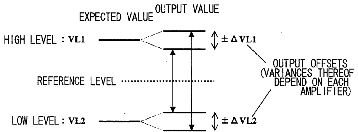
FIG . 16 PRIOR ART
