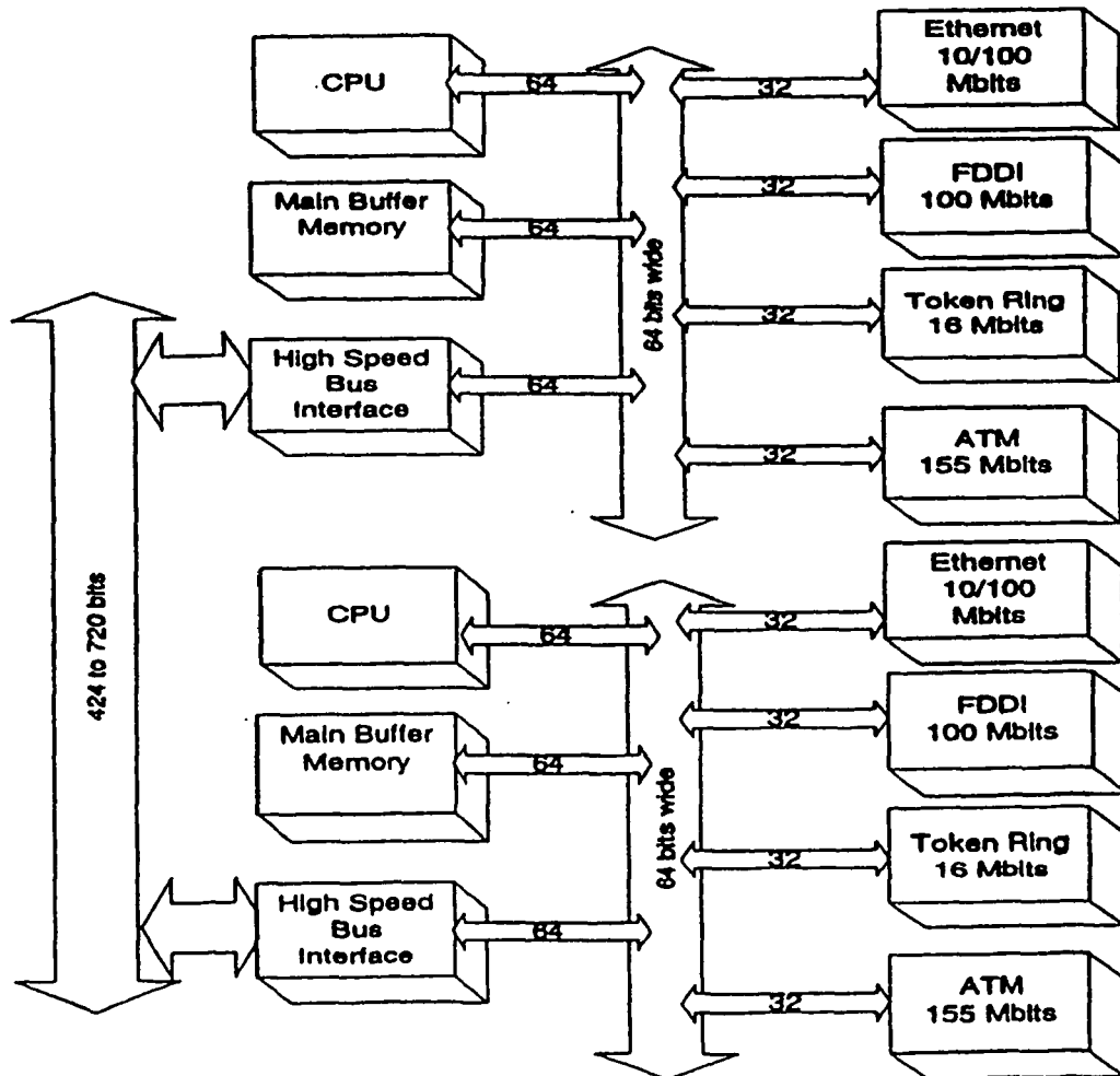
Fig. 5 PRIOR ART
