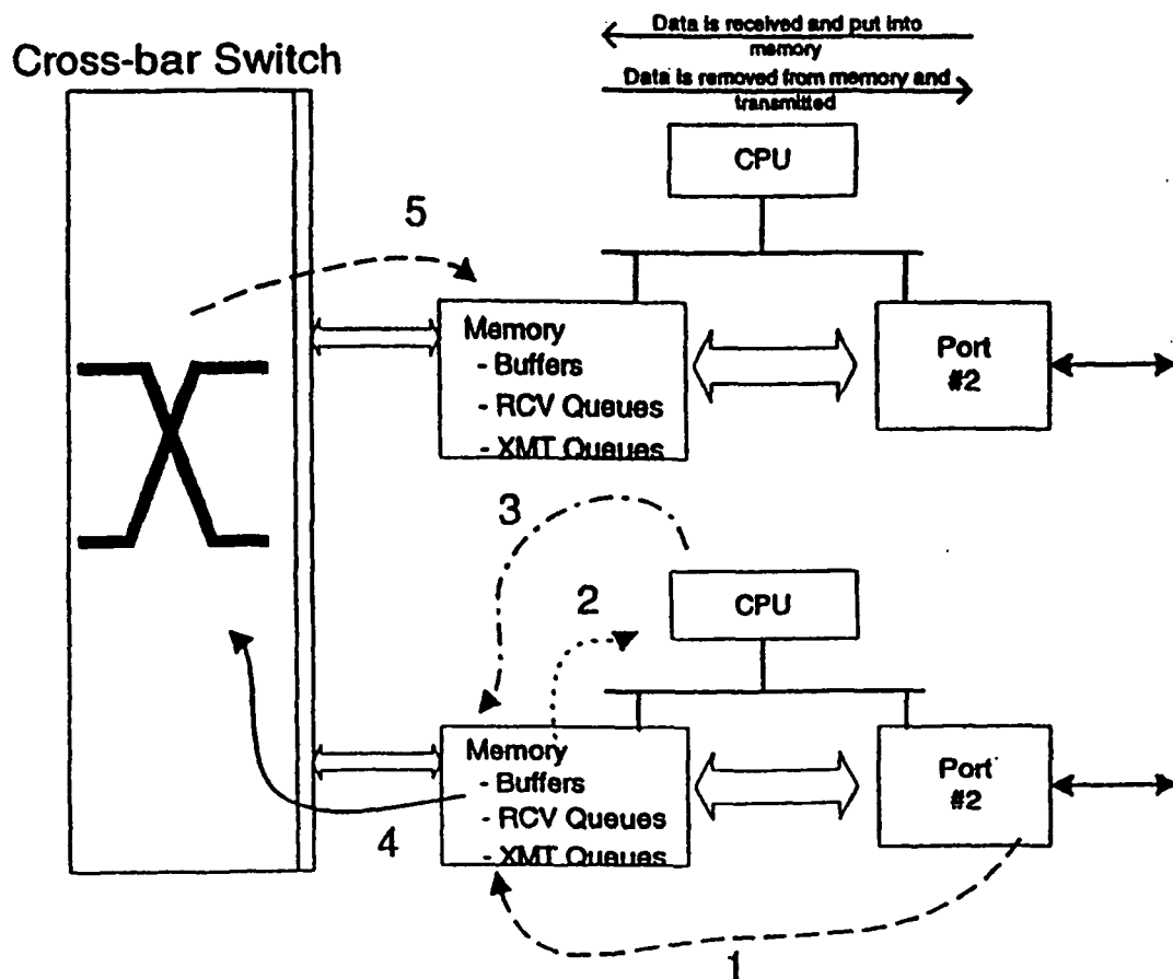
Fig. 8 PRIOR ART
