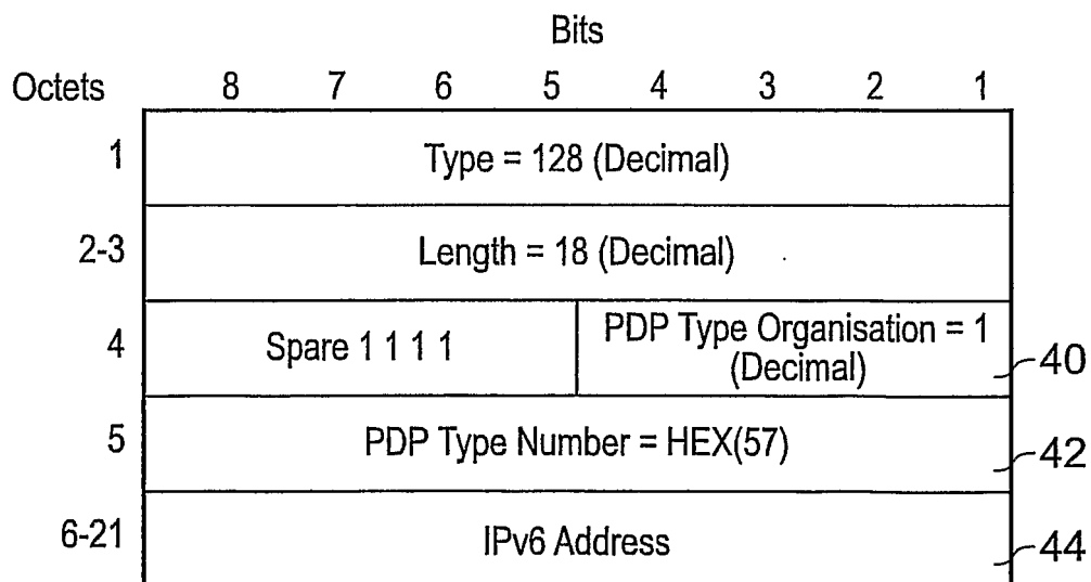
Fig. 9: End User Address Information Element for IPv6
