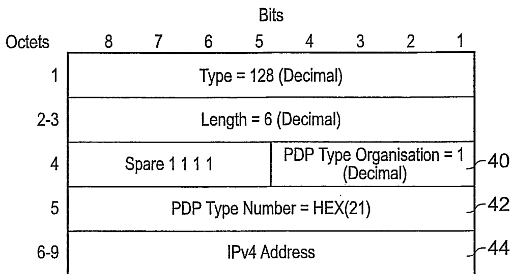
Fig. 8: End User Address Information Element for IPv4
