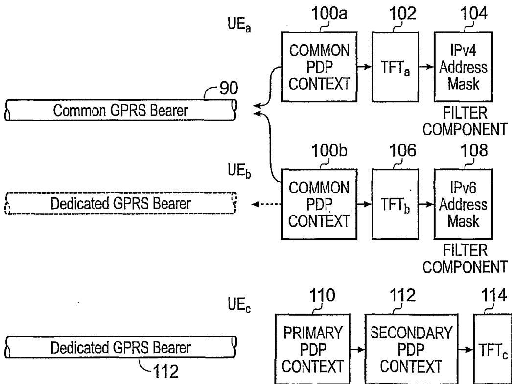
Fig. 13: TFT for Common PDP Context
