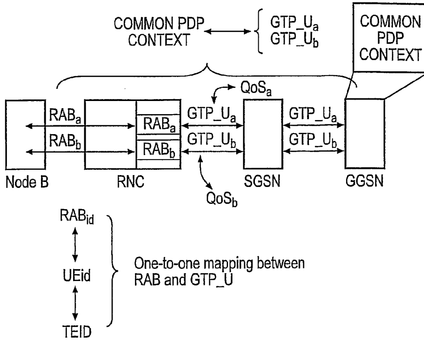
Fig. 14: Common PDP Context Different GPRS Bearer
