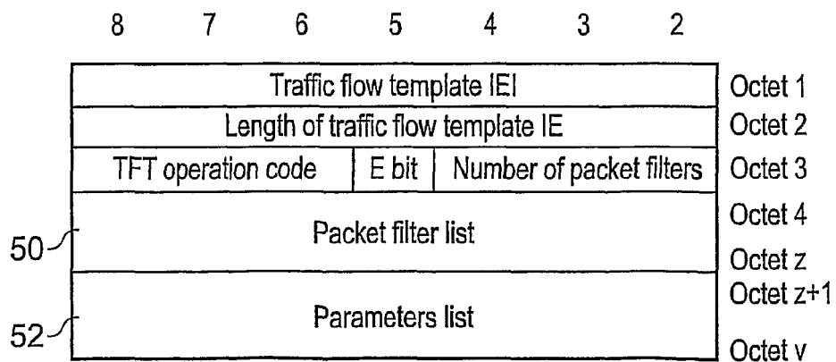
Fig. 12: Traffic Flow Template Information Element
