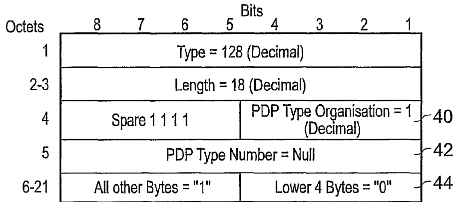
Fig. 11: The End User Address Information Element for Common PDP Context IPv4
