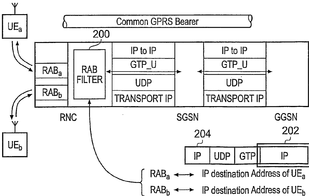
Fig. 15: Common PDP Context Shared GTP_U
