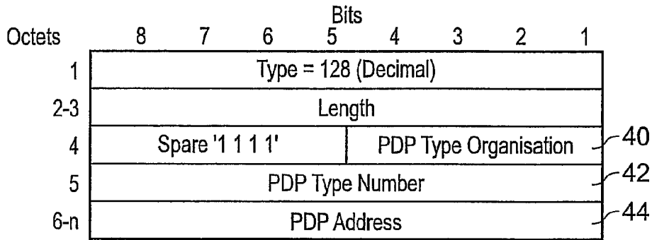
Fig. 6: End User Address Information Element
