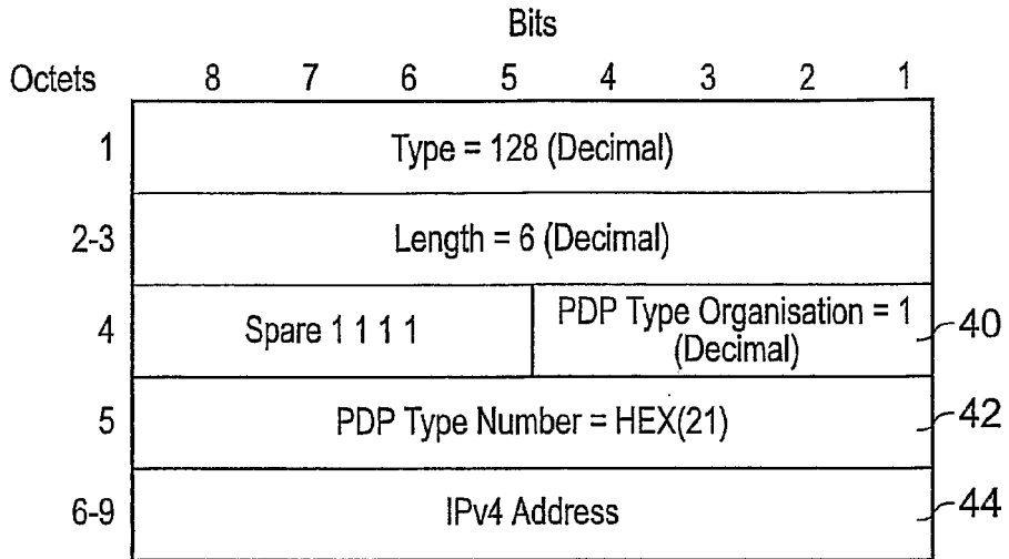
Fig. 8: End User Address Information Element for IPv4
