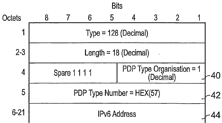
Fig. 9: End User Address Information Element for IPv6
