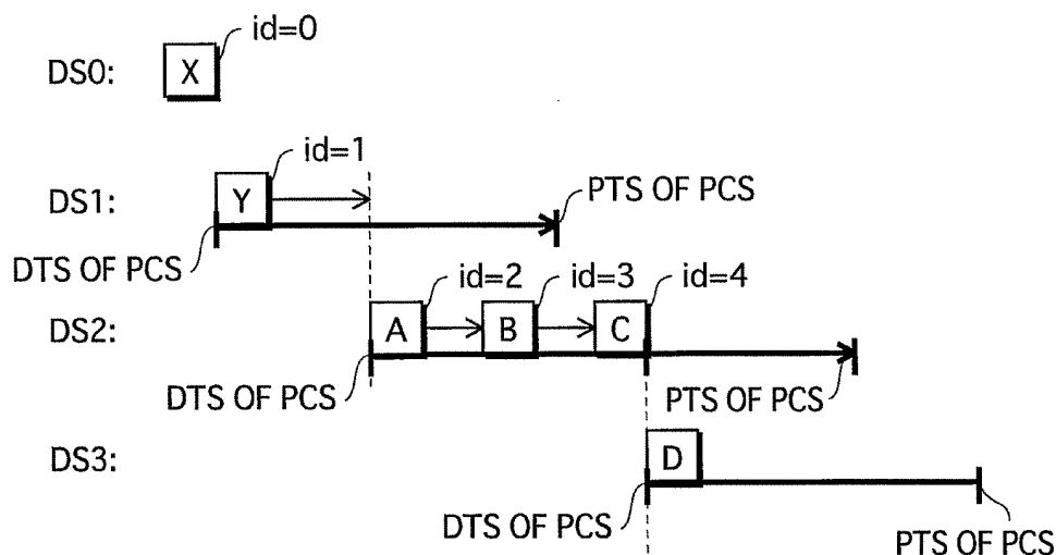
FIG.27B ACTIVE PERIOD OVERLAPPING AND ODS TRANSFER
