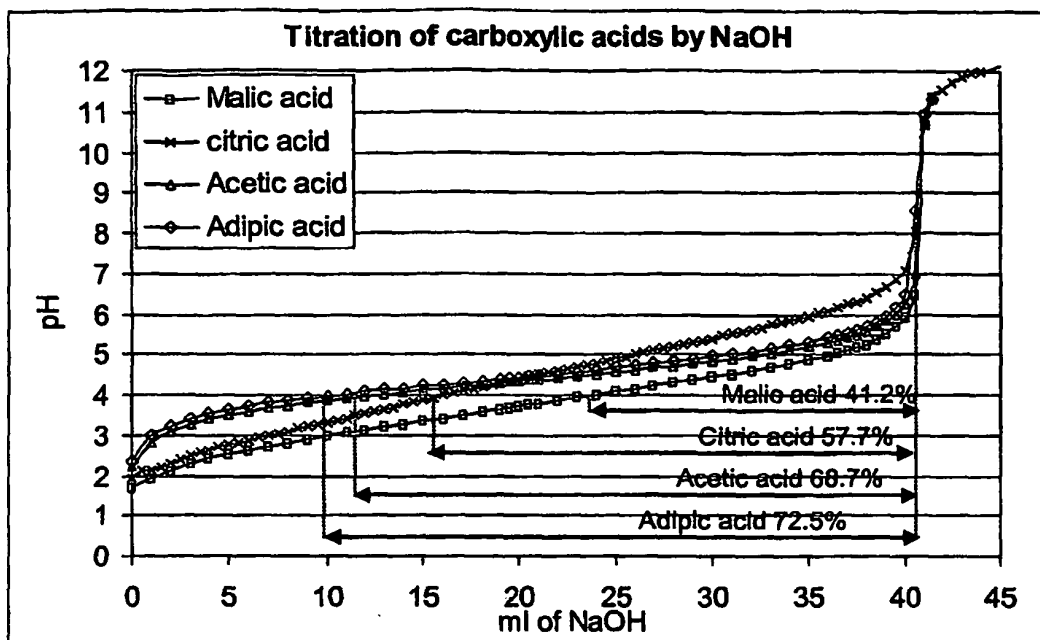
FIG. 1 Standard acid base titration curves of four carboxylates
