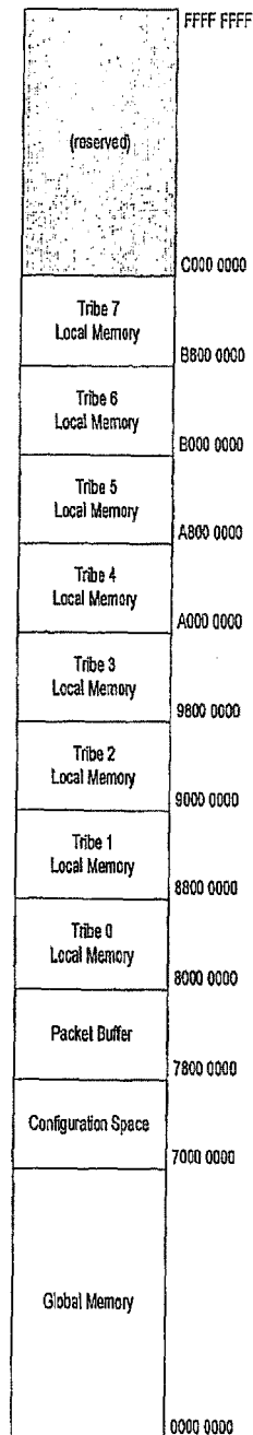
Fig. 2 - Memory Map
