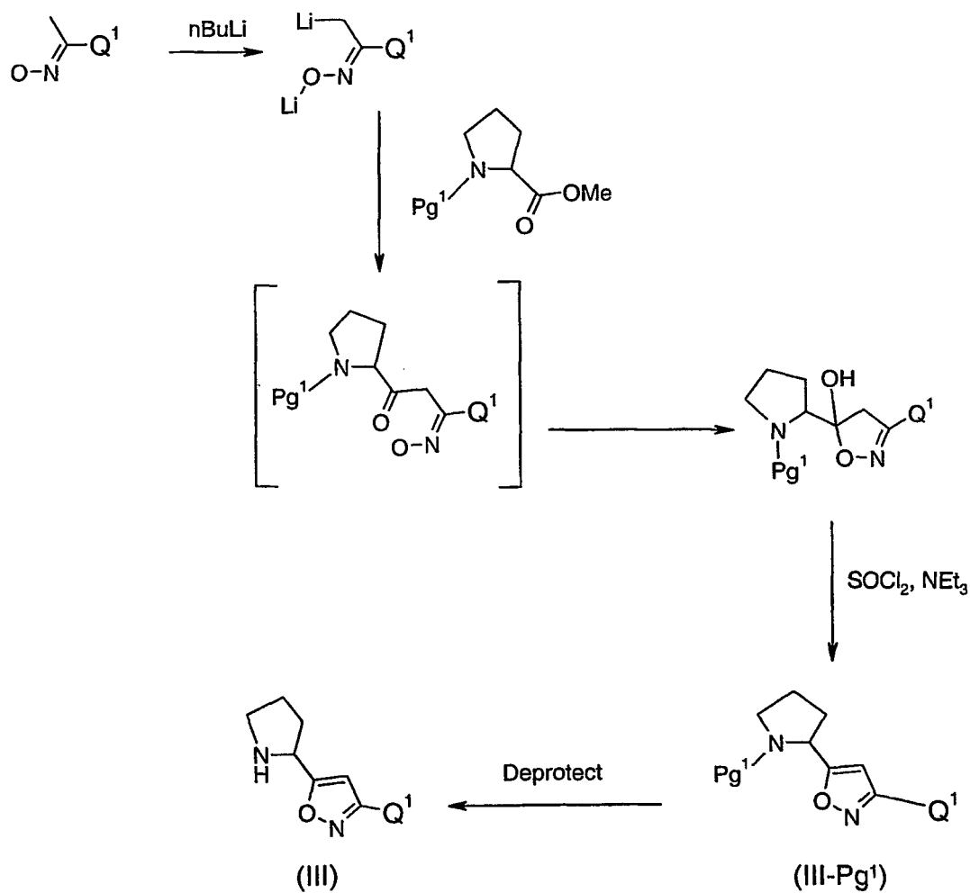
Reaction Scheme 1
