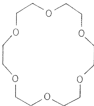
18-CROWN-6
