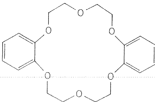
DIBENZOYL-18-CROWN-6
