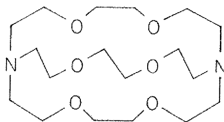
CRYPTAND [2.2.2]
