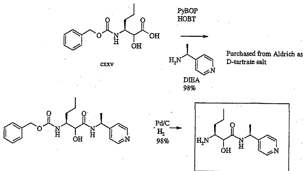
SCHEME 10
