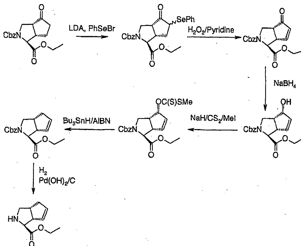
SCHEME 3
