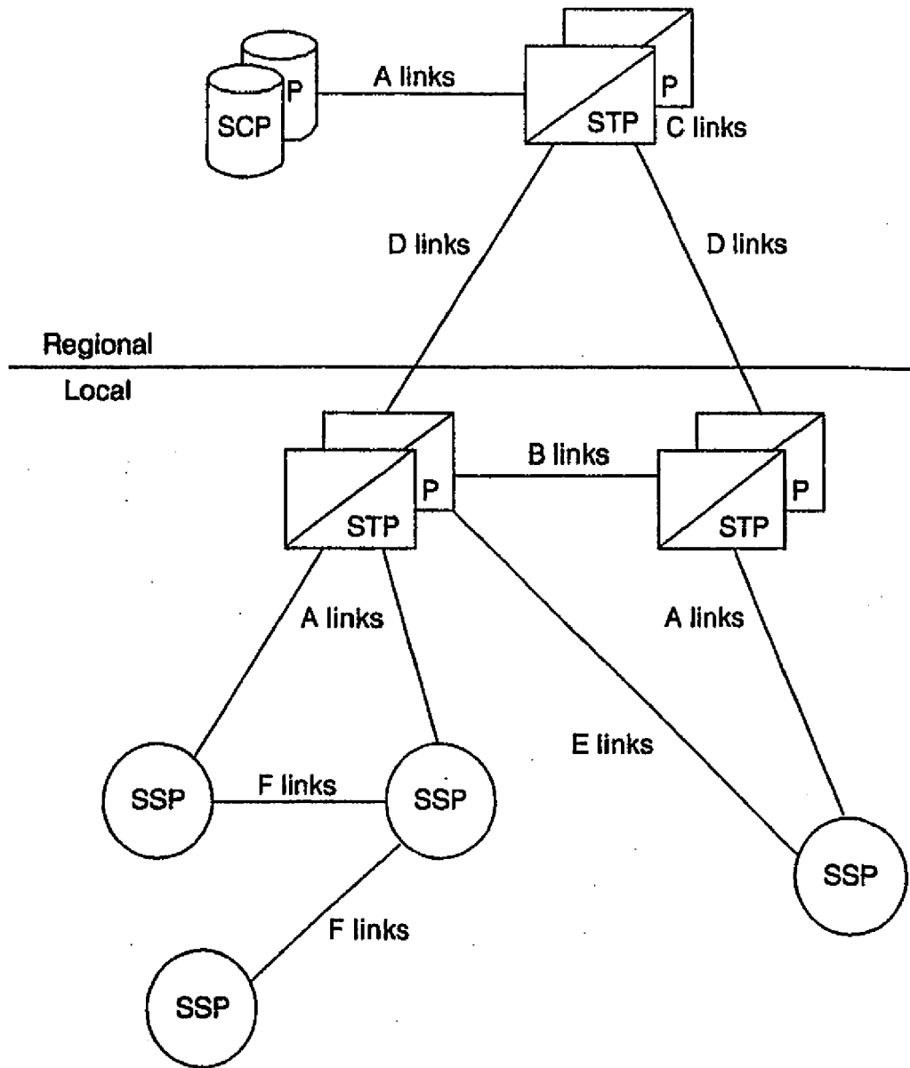
FIG. 7 PRIOR ART
