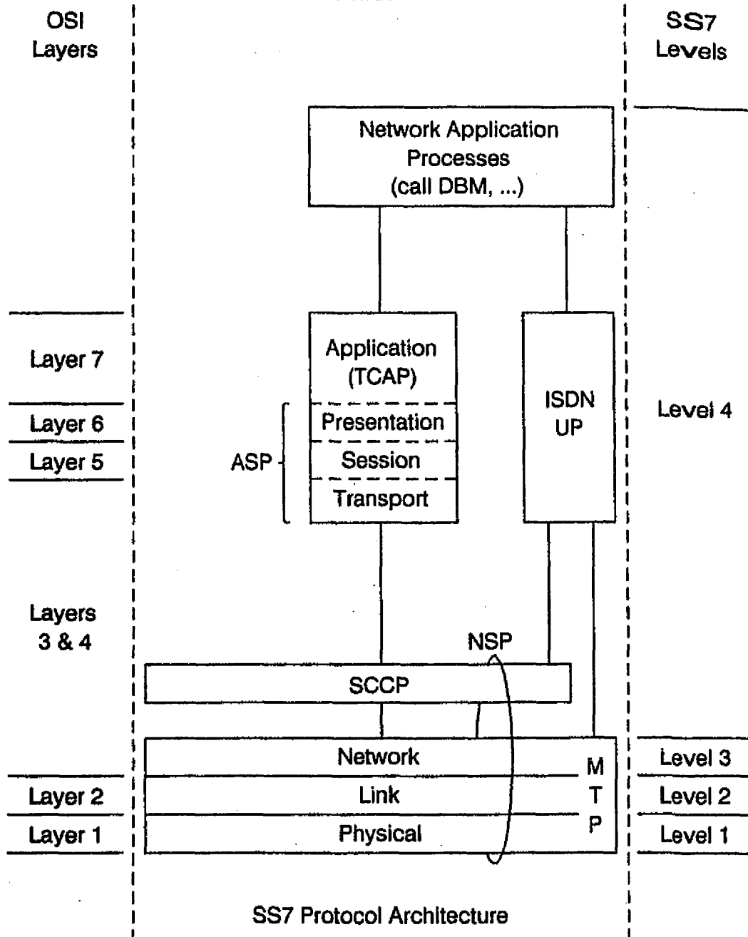
FIG. 8 PRIOR ART
