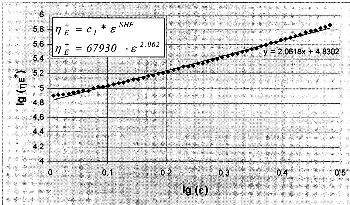
Figure 1: Determination of the SHI of WB130HMS at a strain rate of 0.1\text{s}^{-1} (SHI@ 0.1\text{s}^{-1} )
