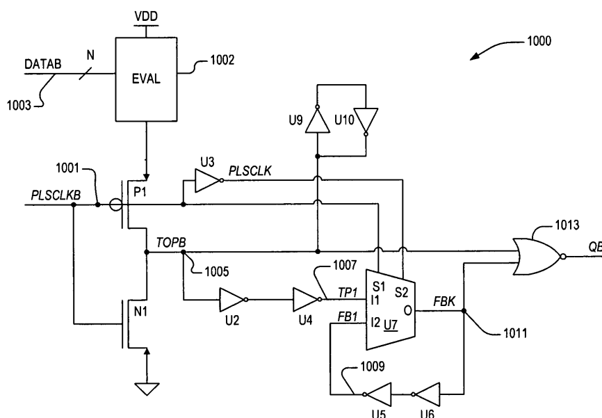
ACCELERATED P-CHANNEL DYNAMIC REGISTER
