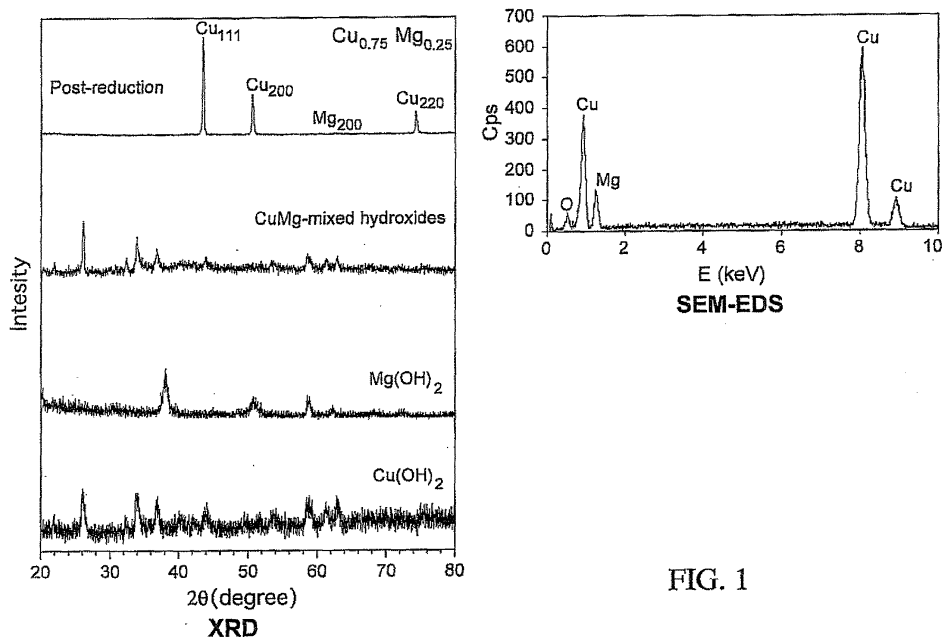
Characterization of \text{Cu}_{0.75}\text{Mg}_{0.25} Nanoalloy 1
