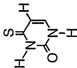
4-thiouracil
