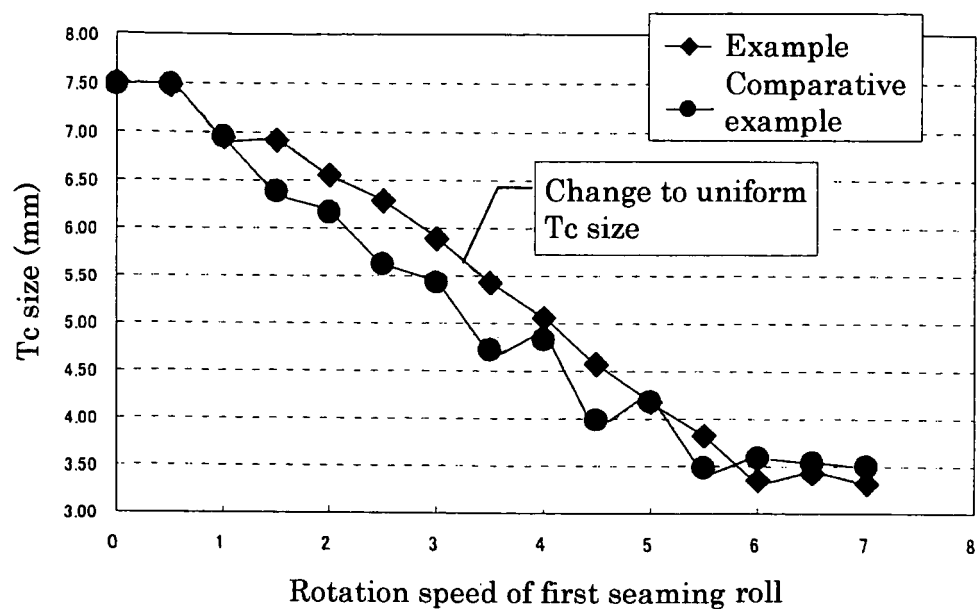
Fig. 16 Relationship between advancement of seaming process and change in Tc size
