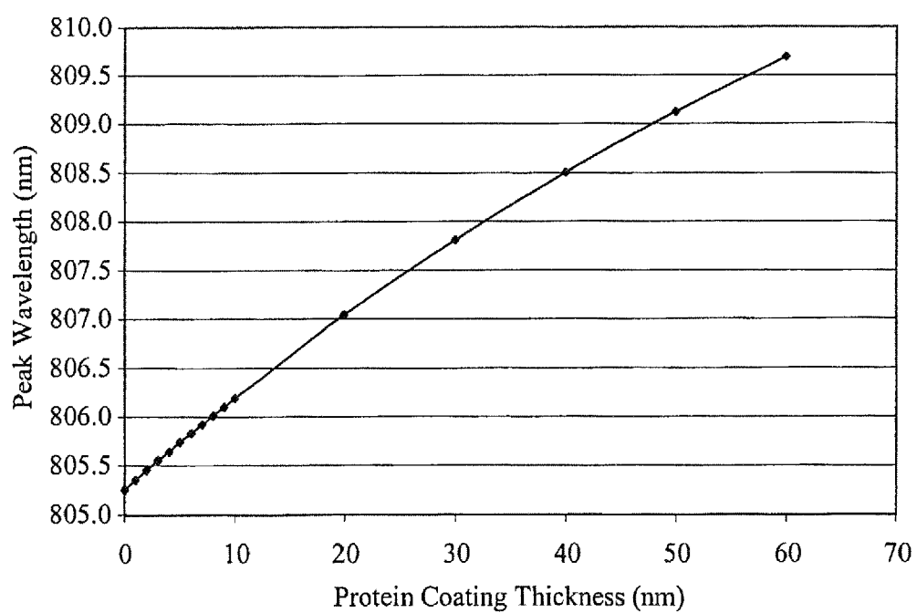
Resonant Peak Wavelength Dependence on Deposited Protein Thickness
