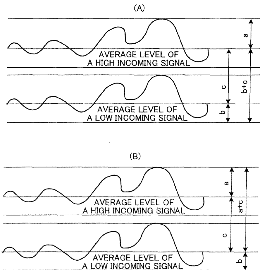
FIG. 9 PRIOR ART
