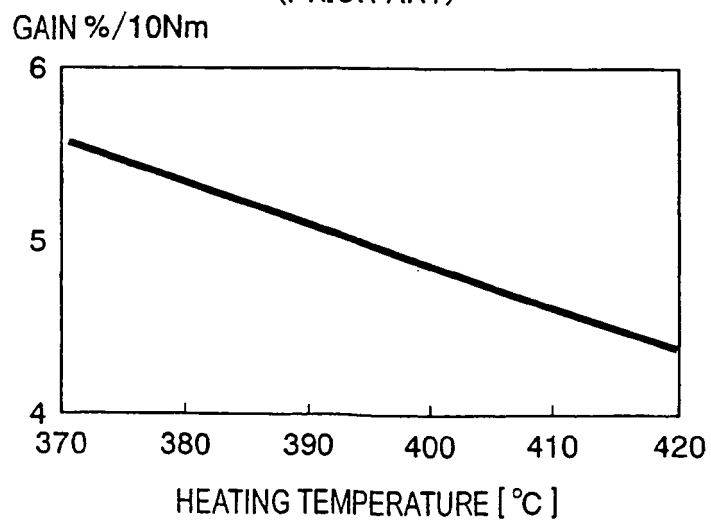
FIG.21 (PRIOR ART)
