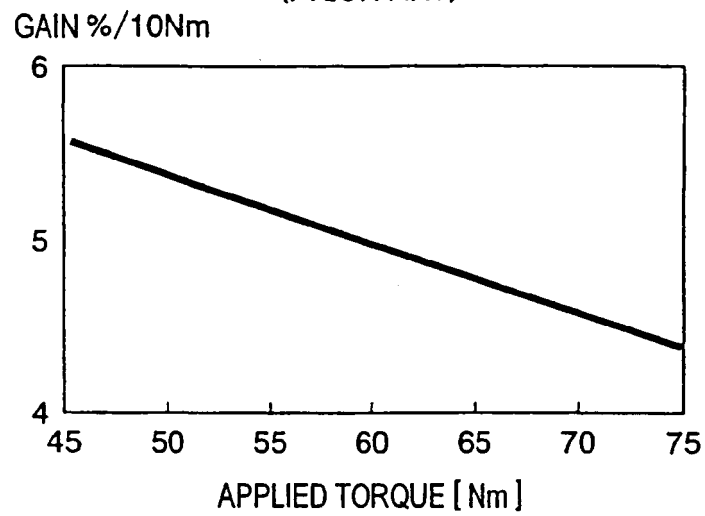
FIG.20 (PRIOR ART)
