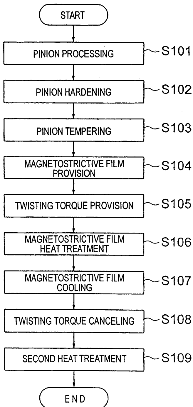
FIG.19 (PRIOR ART)
