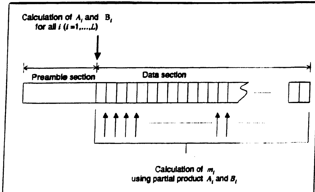
Figure 11 - Partial H_s pre-calculation.
